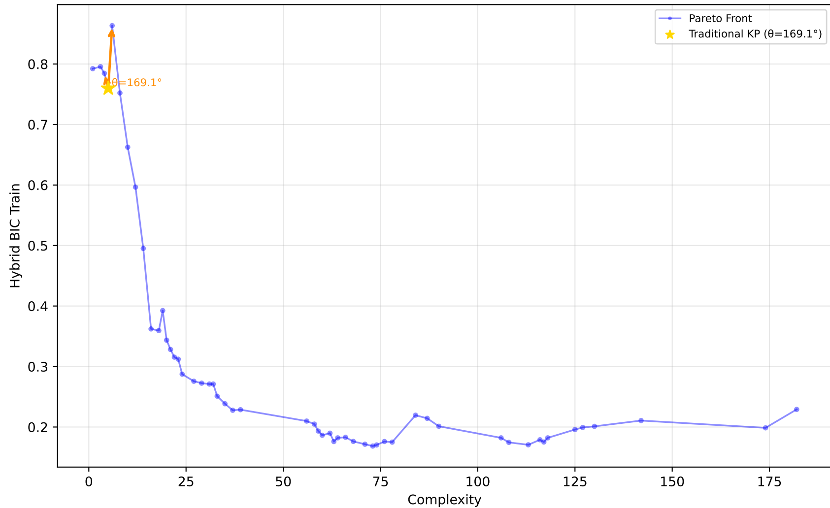
561_cpu - Run 11 - SVP - Hybrid BIC Train \lambda_1=0.90, \lambda_2=0.00, \lambda_3=0.30 | Difficulty: 1.00 | Method: hmr
