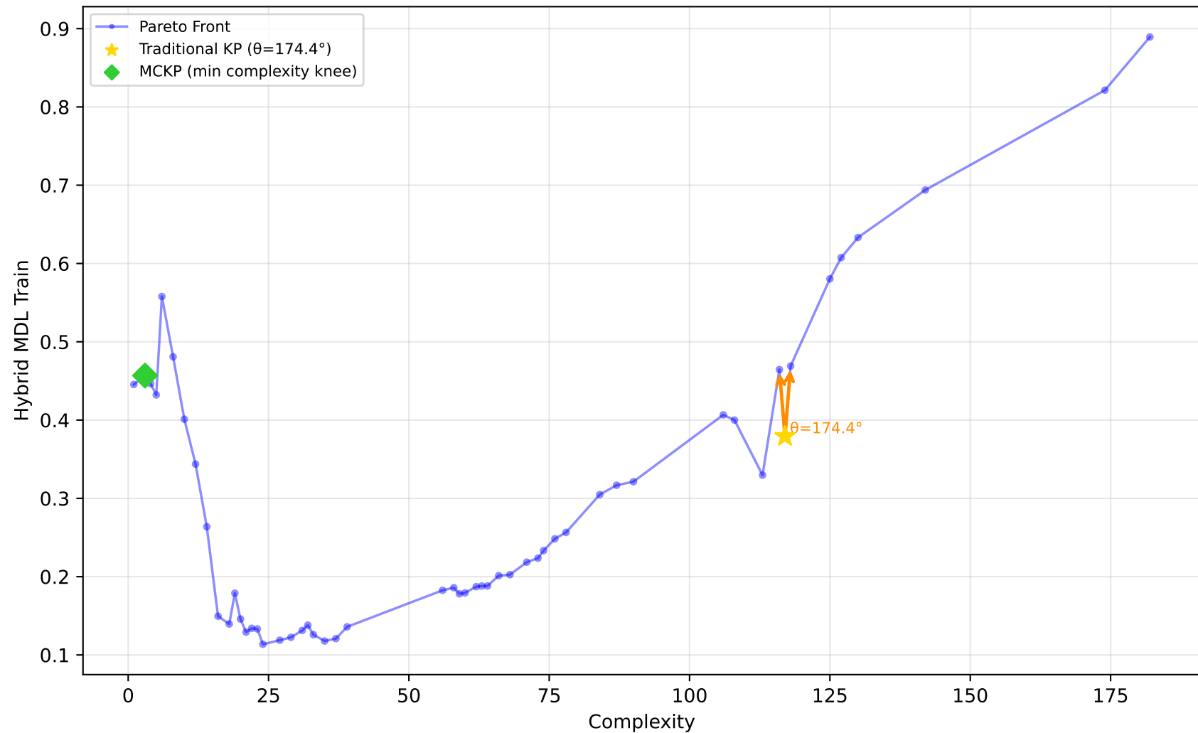
561_cpu - Run 11 - SVP - Hybrid MDL Train \lambda_1=0.90, \lambda_2=0.00, \lambda_3=0.30 | Difficulty: 1.00 | Method: hmr
