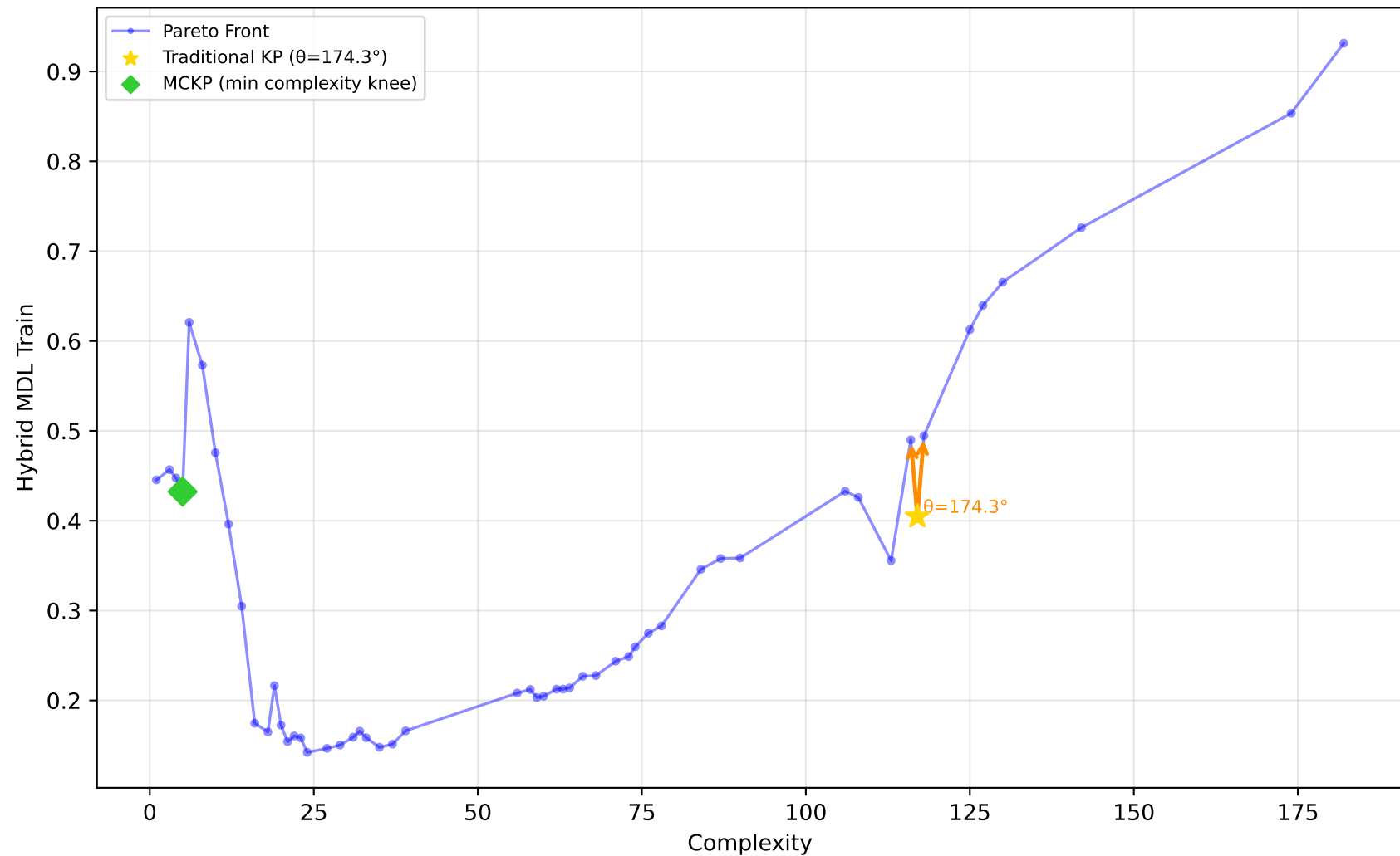
561_cpu - Run 11 - SVP - Hybrid MDL Train \lambda_1=1.00, \lambda_2=0.00, \lambda_3=0.40 | Difficulty: 1.00 | Method: hmr
