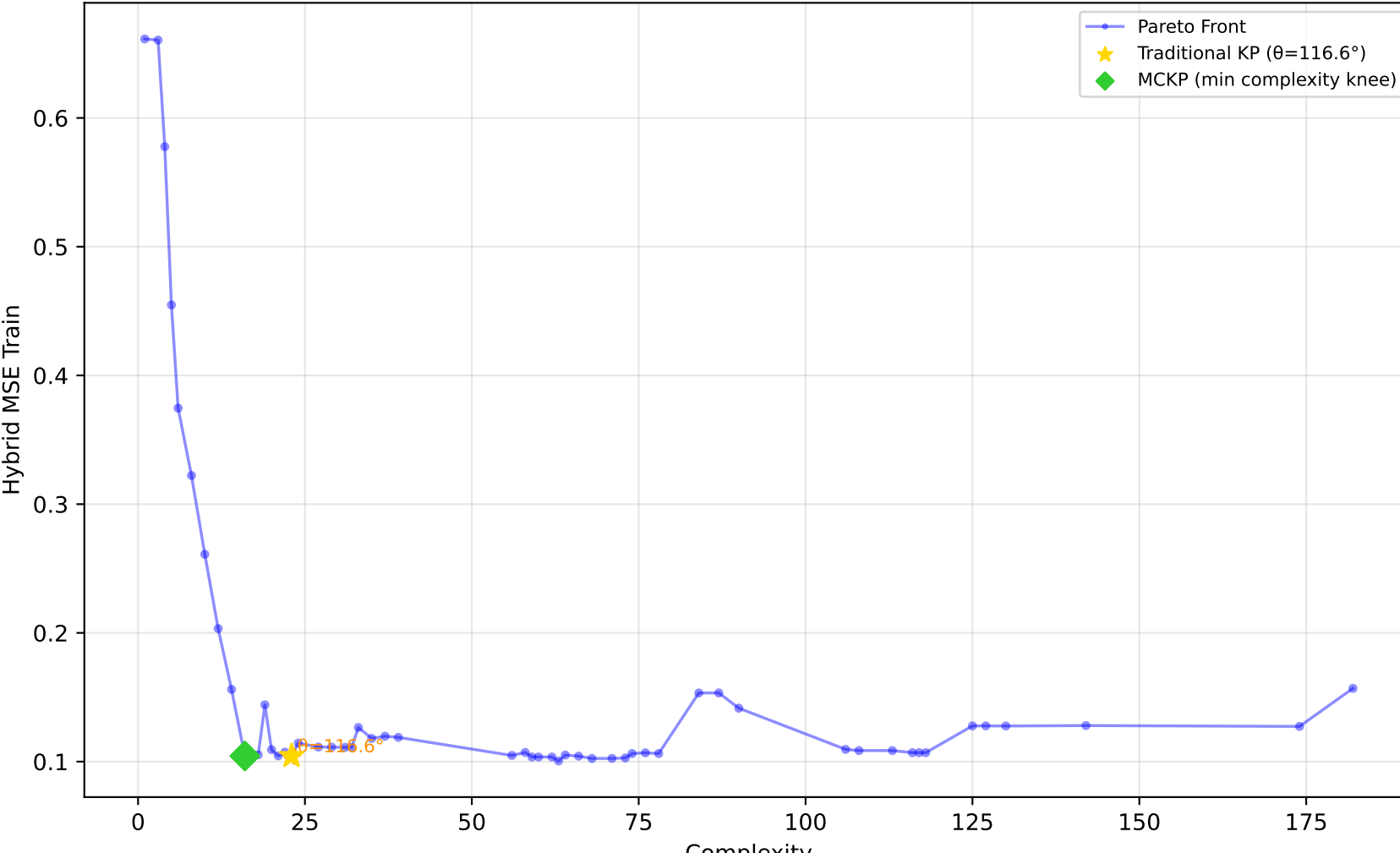
561_cpu - Run 11 - SVP - Hybrid MSE Train \lambda_1=0.90, \lambda_2=0.00, \lambda_3=0.30 | Difficulty: 1.00 | Method: hmr
