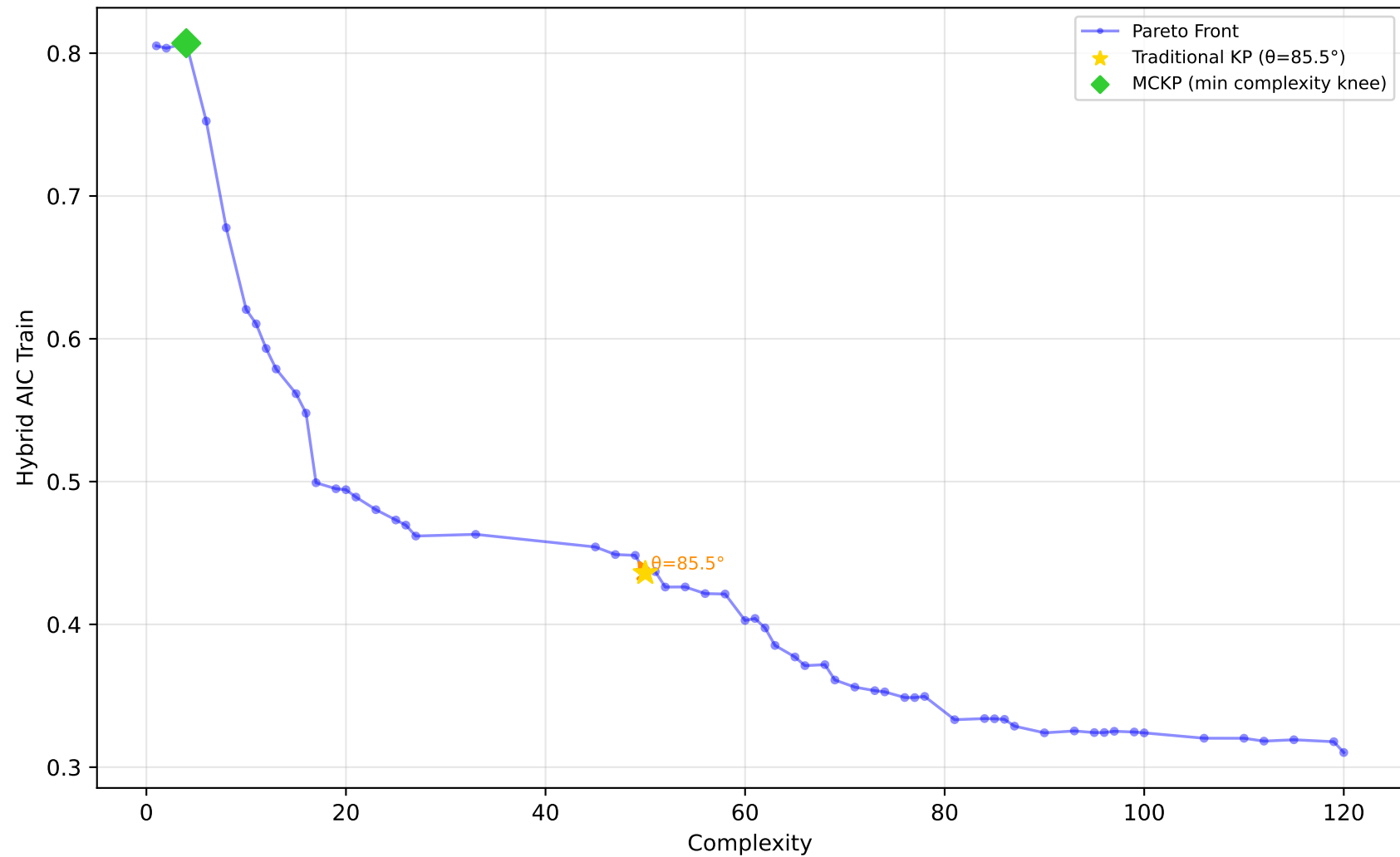
561_cpu - Run 12 - MVP - Hybrid AIC Train \lambda_1=0.50, \lambda_2=0.20, \lambda_3=0.00 | Difficulty: 1.00 | Method: hmr
