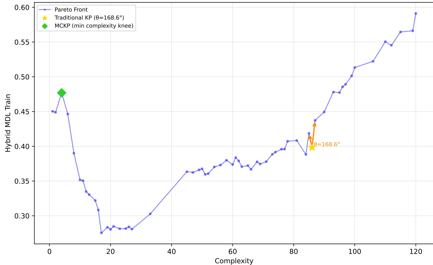
561_cpu - Run 12 - MVP - Hybrid MDL Train \lambda_1=0.50, \lambda_2=0.20, \lambda_3=0.00 | Difficulty: 1.00 | Method: hmr
