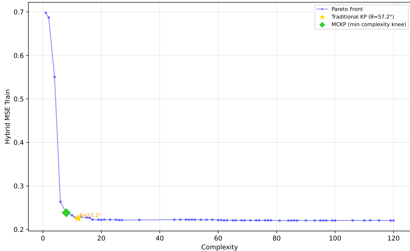
561_cpu - Run 12 - MVP - Hybrid MSE Train \lambda_1=0.50, \lambda_2=0.20, \lambda_3=0.00 | Difficulty: 1.00 | Method: hmr
