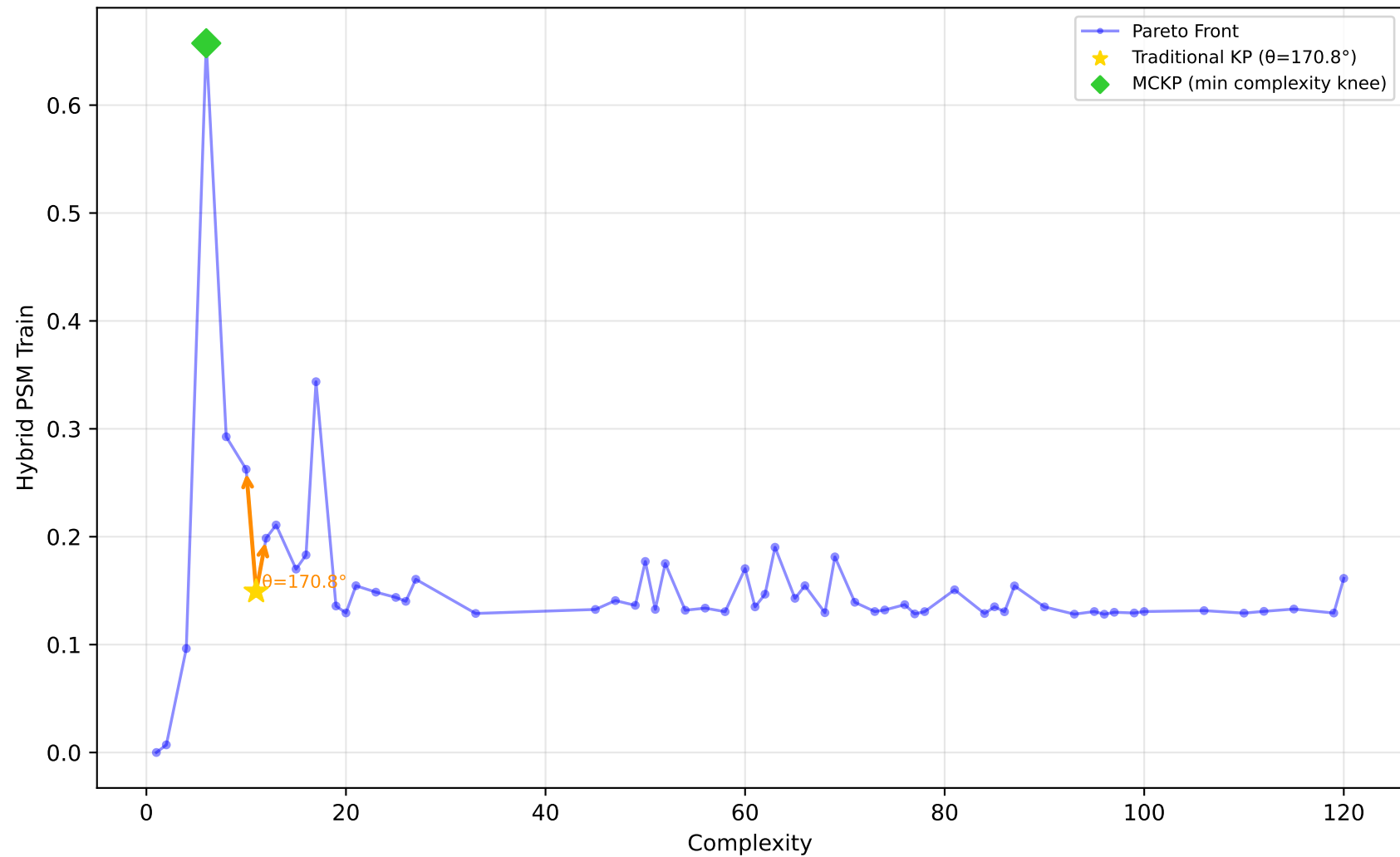
561_cpu - Run 12 - MVP - Hybrid PSM Train \lambda_1=0.70, \lambda_2=0.00, \lambda_3=0.10 | Difficulty: 1.00 | Method: hmr
