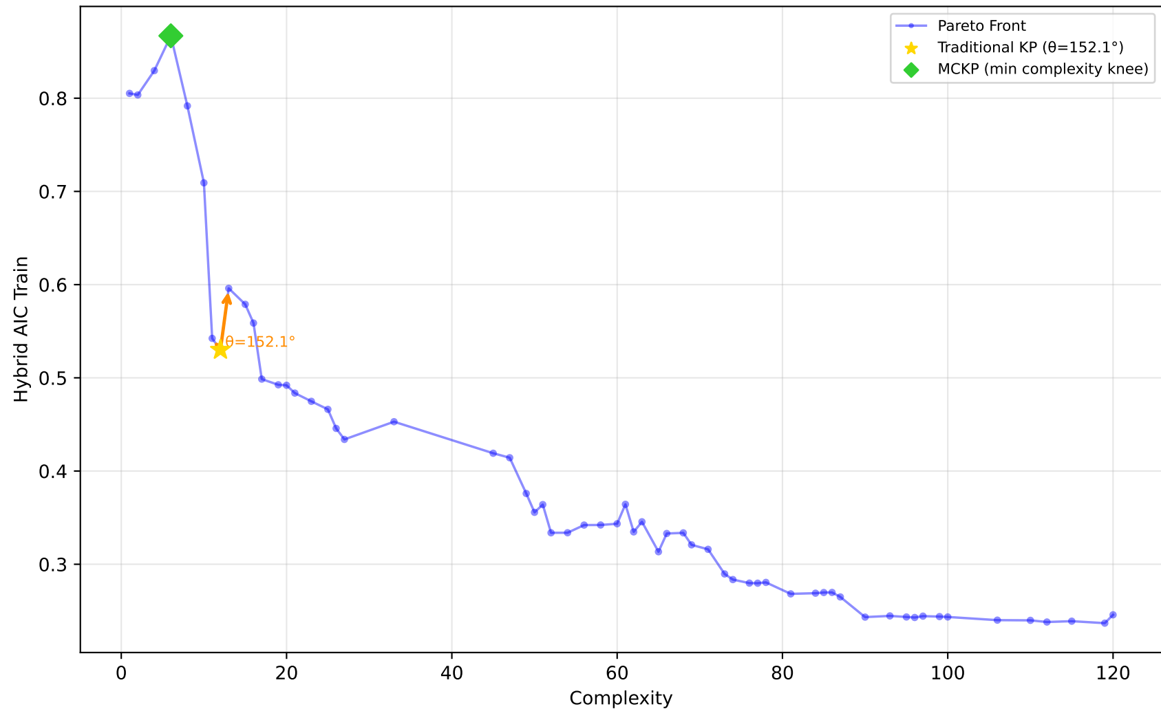
561_cpu - Run 12 - SVP - Hybrid AIC Train \lambda_1=0.90, \lambda_2=0.00, \lambda_3=0.30 | Difficulty: 1.00 | Method: hmr
