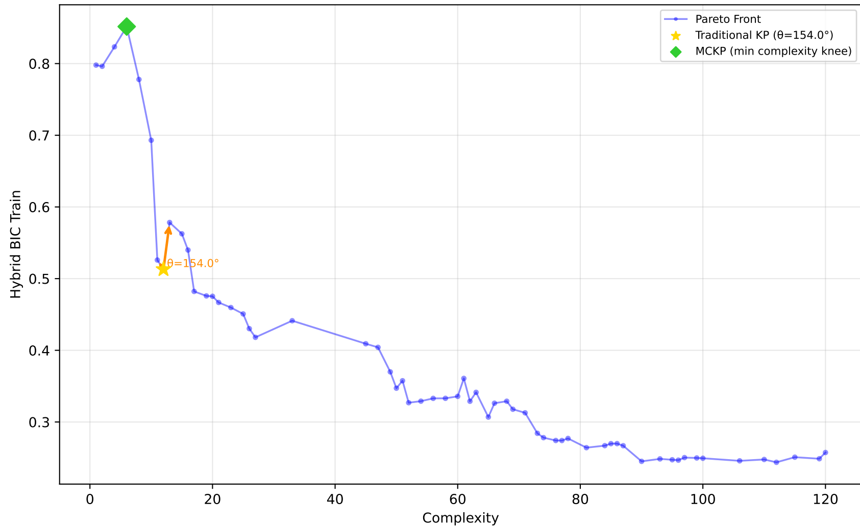
561_cpu - Run 12 - SVP - Hybrid BIC Train \lambda_1=0.90, \lambda_2=0.00, \lambda_3=0.30 | Difficulty: 1.00 | Method: hmr
