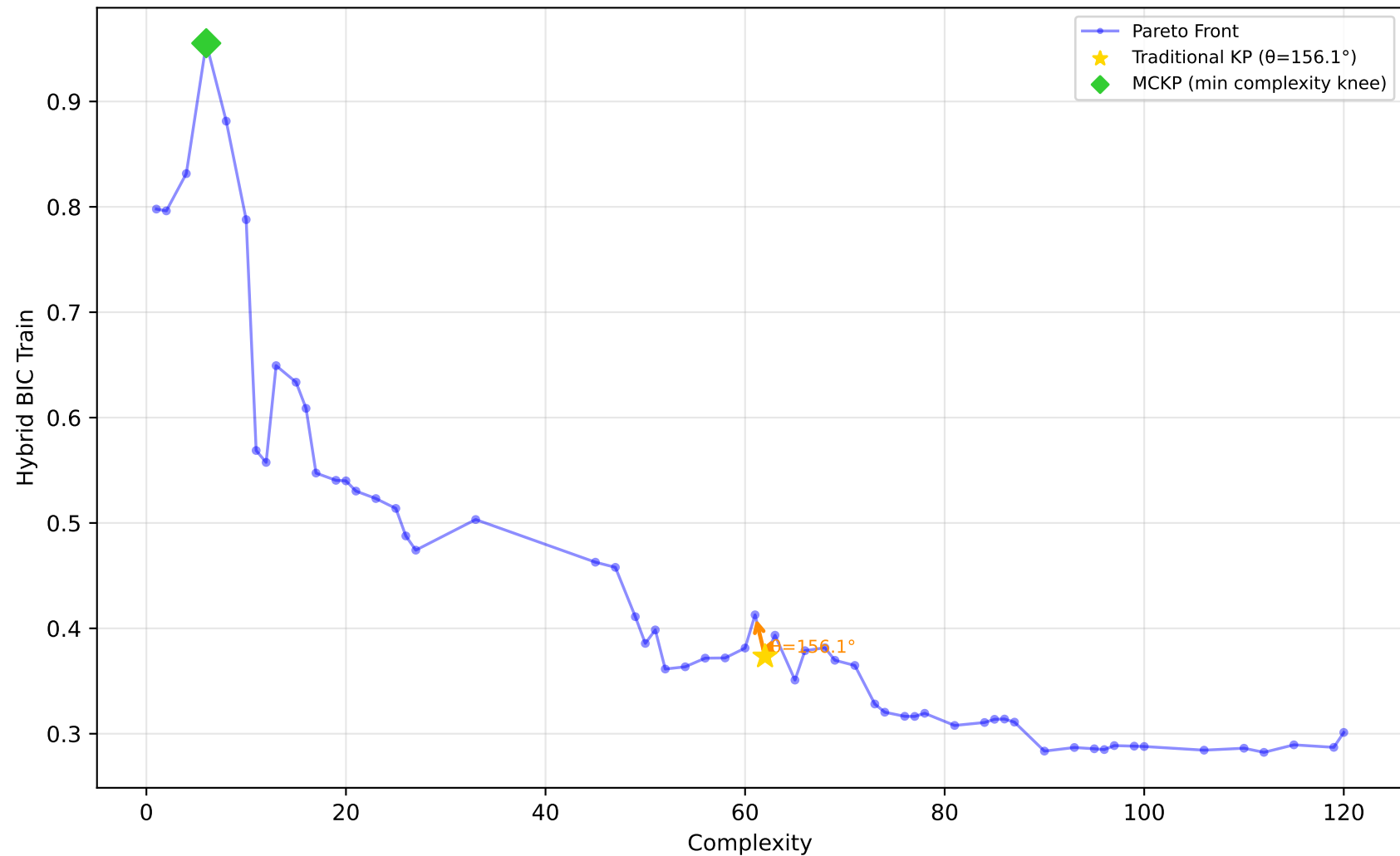
561_cpu - Run 12 - SVP - Hybrid BIC Train \lambda_1=1.00, \lambda_2=0.00, \lambda_3=0.40 | Difficulty: 1.00 | Method: hmr
