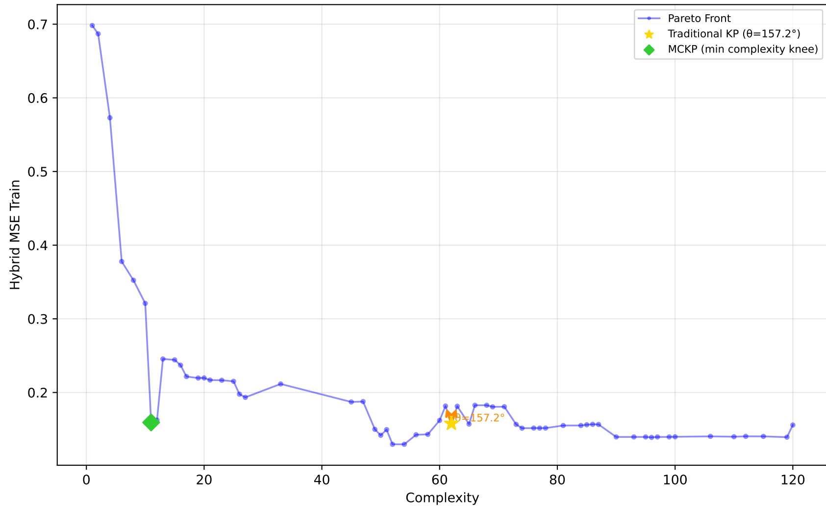
561_cpu - Run 12 - SVP - Hybrid MSE Train \lambda_1=0.90, \lambda_2=0.00, \lambda_3=0.30 | Difficulty: 1.00 | Method: hmr
