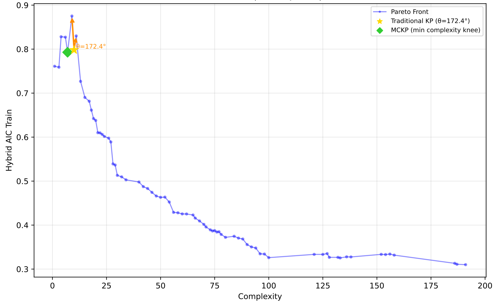
561_cpu - Run 13 - MVP - Hybrid AIC Train \lambda_1=0.50, \lambda_2=0.20, \lambda_3=0.00 | Difficulty: 1.00 | Method: hmr
