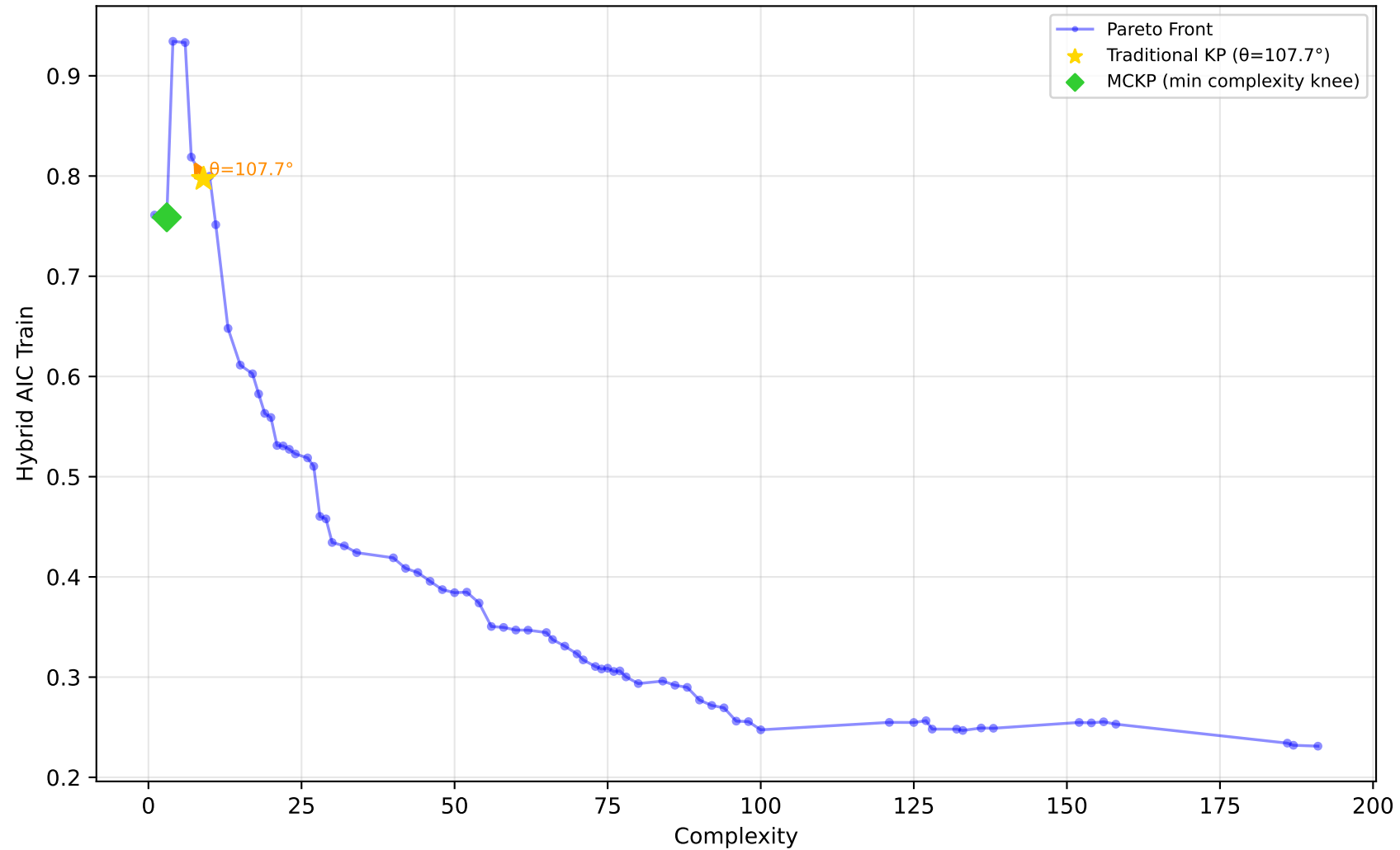
561_cpu - Run 13 - MVP - Hybrid AIC Train \lambda_1=0.70, \lambda_2=0.00, \lambda_3=0.10 | Difficulty: 1.00 | Method: hmr
