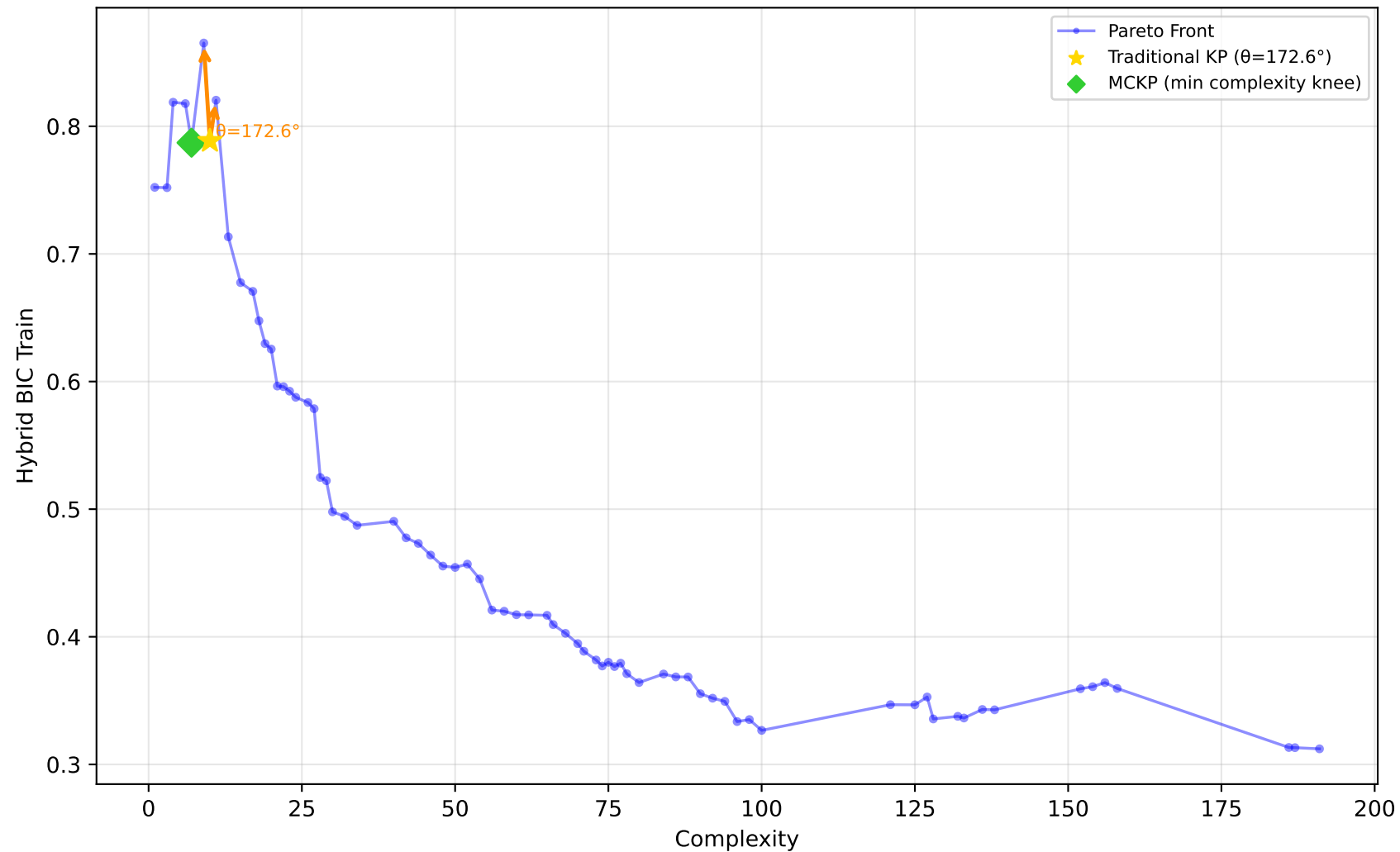
561_cpu - Run 13 - MVP - Hybrid BIC Train \lambda_1=0.50, \lambda_2=0.20, \lambda_3=0.00 | Difficulty: 1.00 | Method: hmr
