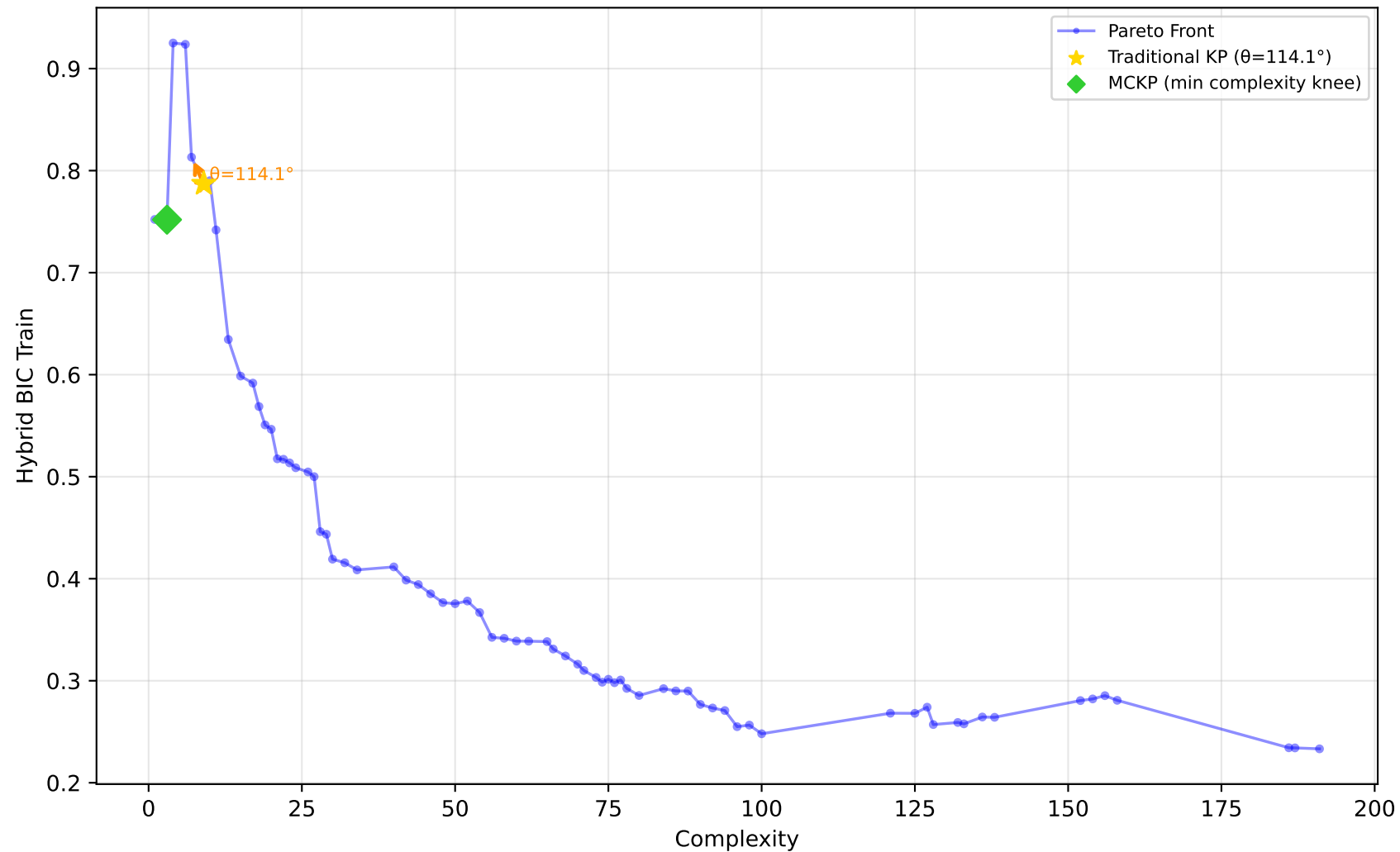
561_cpu - Run 13 - MVP - Hybrid BIC Train \lambda_1=0.70, \lambda_2=0.00, \lambda_3=0.10 | Difficulty: 1.00 | Method: hmr
