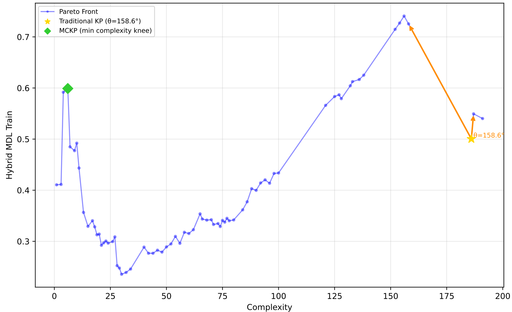
561_cpu - Run 13 - MVP - Hybrid MDL Train \lambda_1=0.70, \lambda_2=0.00, \lambda_3=0.10 | Difficulty: 1.00 | Method: hmr
