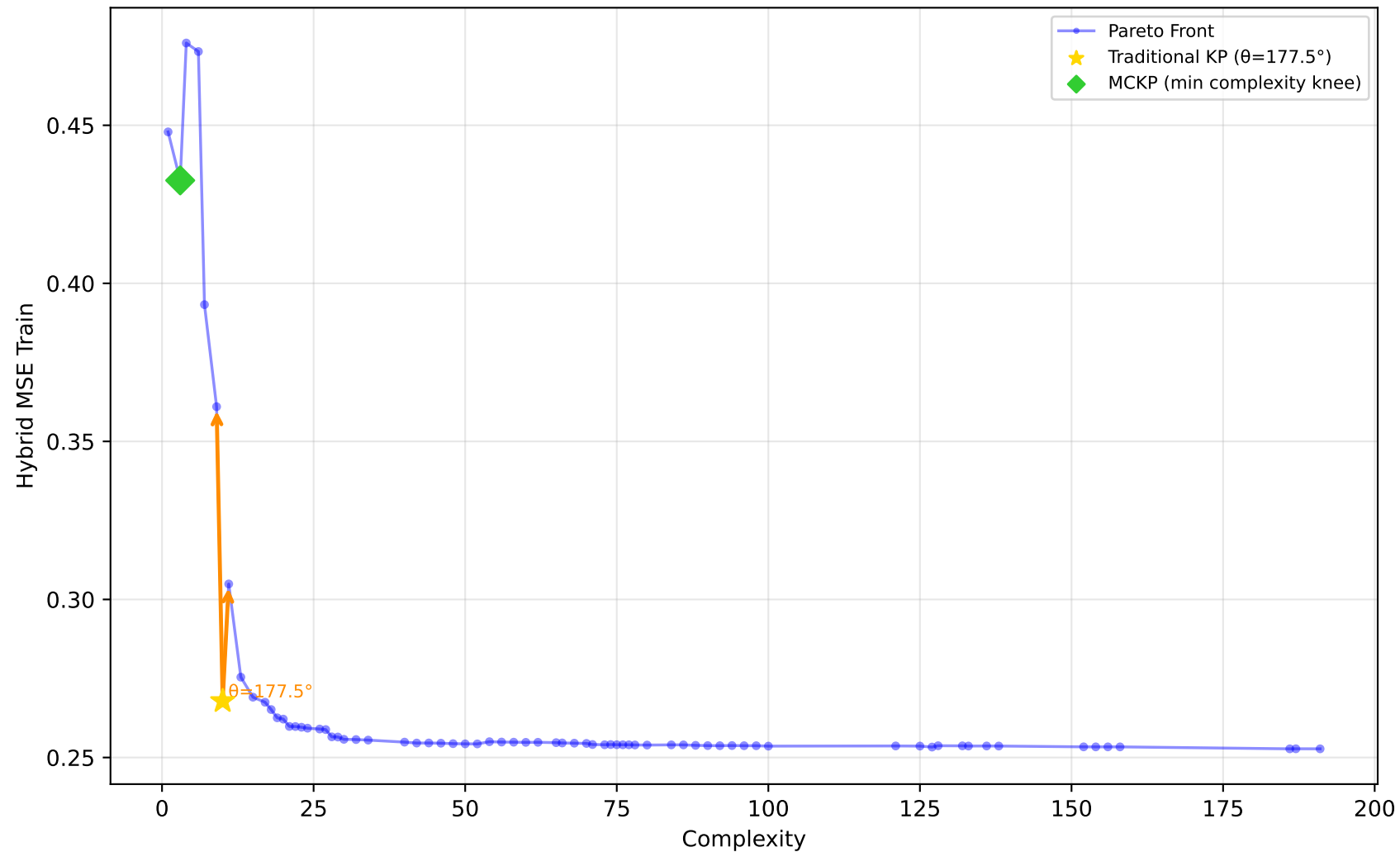
561_cpu - Run 13 - MVP - Hybrid MSE Train \lambda_1=0.50, \lambda_2=0.20, \lambda_3=0.00 | Difficulty: 1.00 | Method: hmr
