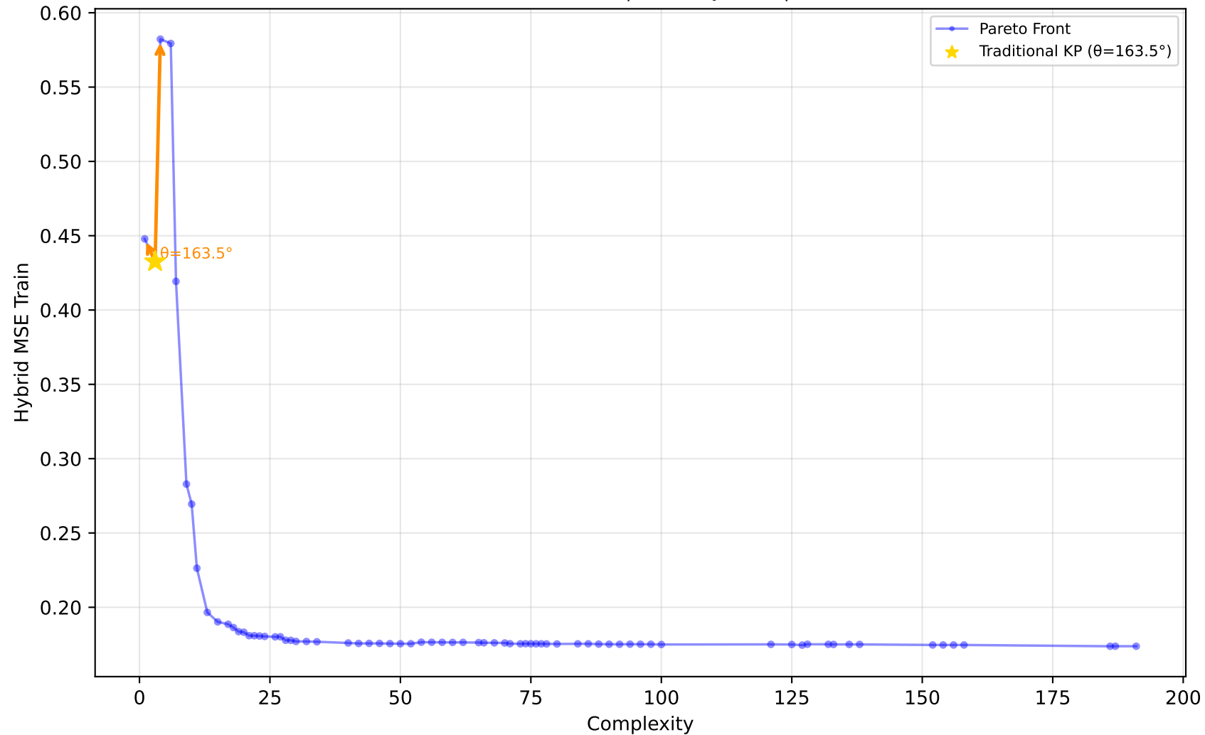
561_cpu - Run 13 - MVP - Hybrid MSE Train \lambda_1=0.70, \lambda_2=0.00, \lambda_3=0.10 | Difficulty: 1.00 | Method: hmr
