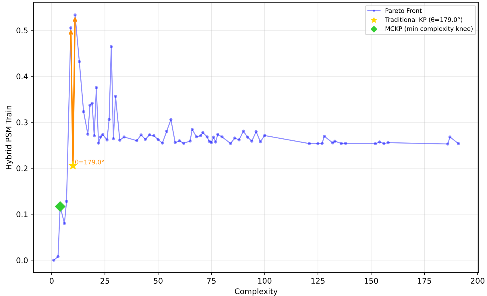
561_cpu - Run 13 - MVP - Hybrid PSM Train \lambda_1=0.50, \lambda_2=0.20, \lambda_3=0.00 | Difficulty: 1.00 | Method: hmr
