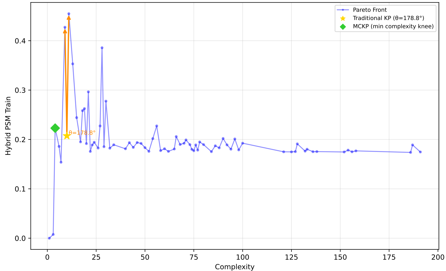
561_cpu - Run 13 - MVP - Hybrid PSM Train \lambda_1=0.70, \lambda_2=0.00, \lambda_3=0.10 | Difficulty: 1.00 | Method: hmr
