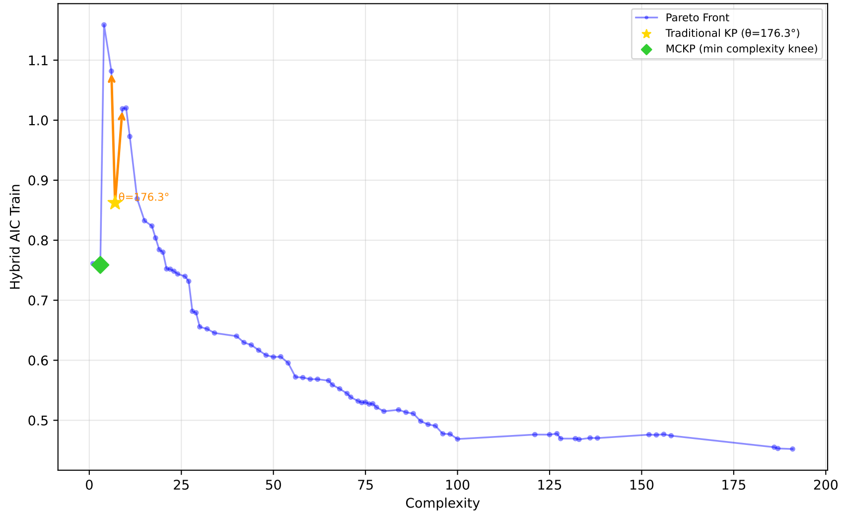
561_cpu - Run 13 - SVP - Hybrid AIC Train \lambda_1=0.90, \lambda_2=0.00, \lambda_3=0.30 | Difficulty: 1.00 | Method: hmr
