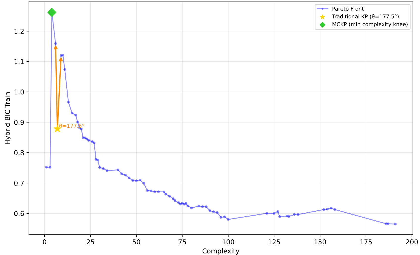
561_cpu - Run 13 - SVP - Hybrid BIC Train \lambda_1=1.00, \lambda_2=0.00, \lambda_3=0.40 | Difficulty: 1.00 | Method: hmr
