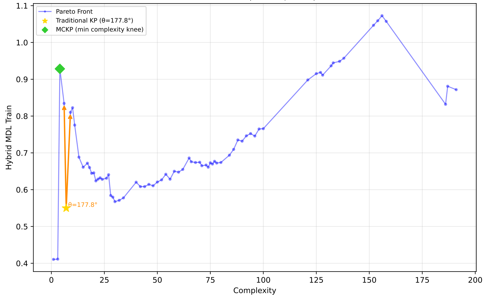
561_cpu - Run 13 - SVP - Hybrid MDL Train \lambda_1=1.00, \lambda_2=0.00, \lambda_3=0.40 | Difficulty: 1.00 | Method: hmr
