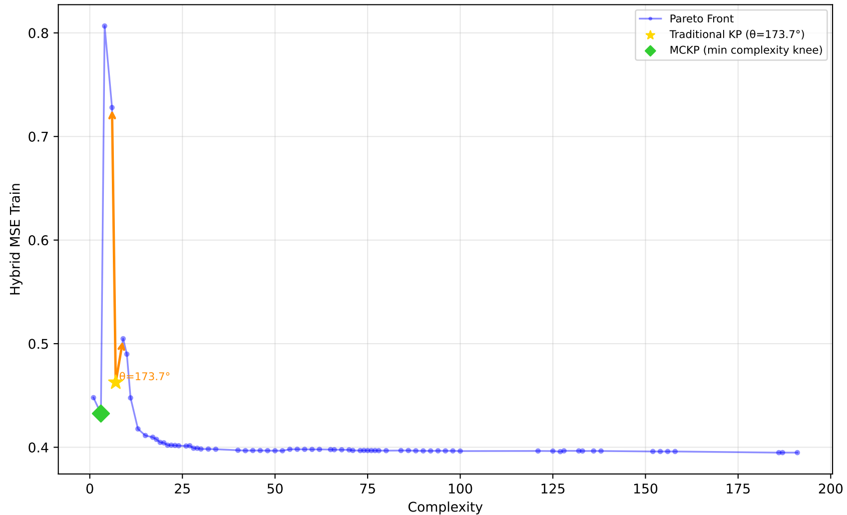
561_cpu - Run 13 - SVP - Hybrid MSE Train \lambda_1=0.90, \lambda_2=0.00, \lambda_3=0.30 | Difficulty: 1.00 | Method: hmr
