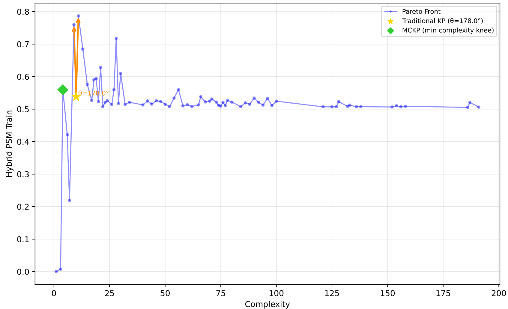
561_cpu - Run 13 - SVP - Hybrid PSM Train \lambda_1=1.00, \lambda_2=0.00, \lambda_3=0.40 | Difficulty: 1.00 | Method: hmr
