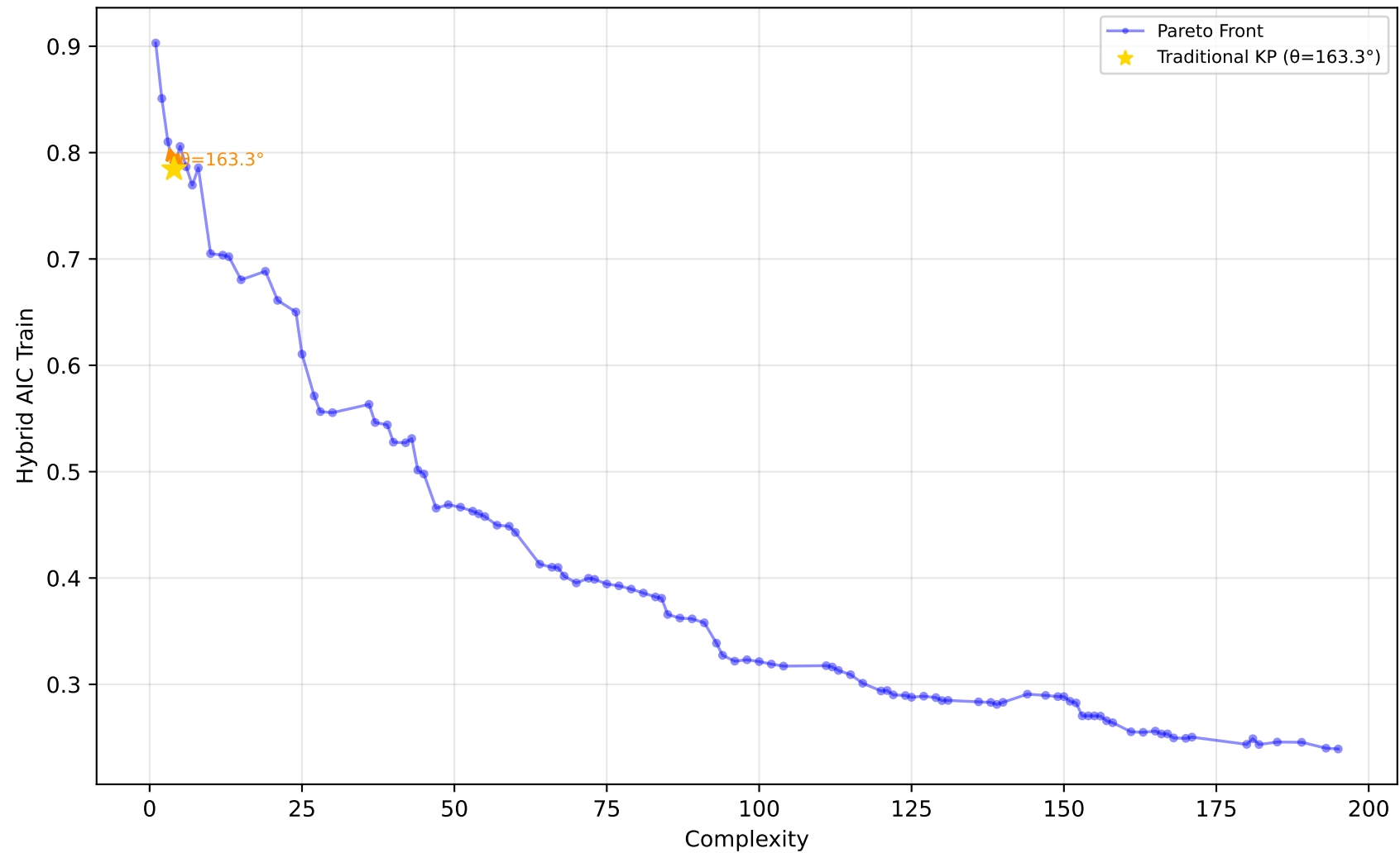
561_cpu - Run 14 - MVP - Hybrid AIC Train \lambda_1=0.70, \lambda_2=0.00, \lambda_3=0.10 | Difficulty: 1.00 | Method: hmr
