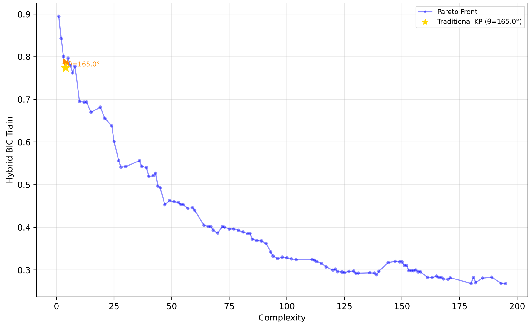
561_cpu - Run 14 - MVP - Hybrid BIC Train \lambda_1=0.70, \lambda_2=0.00, \lambda_3=0.10 | Difficulty: 1.00 | Method: hmr
