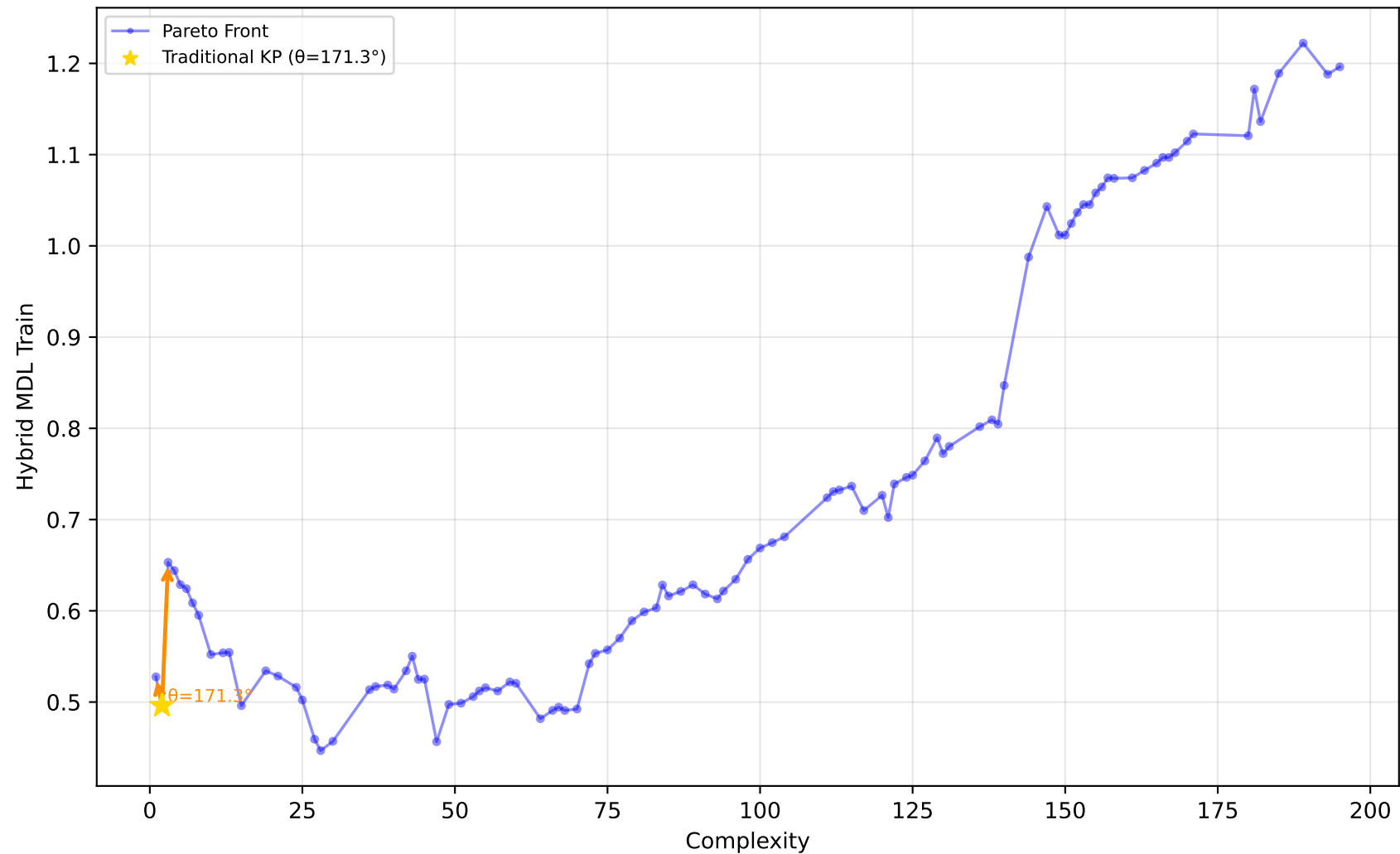
561_cpu - Run 14 - MVP - Hybrid MDL Train \lambda_1=0.50, \lambda_2=0.20, \lambda_3=0.00 | Difficulty: 1.00 | Method: hmr
