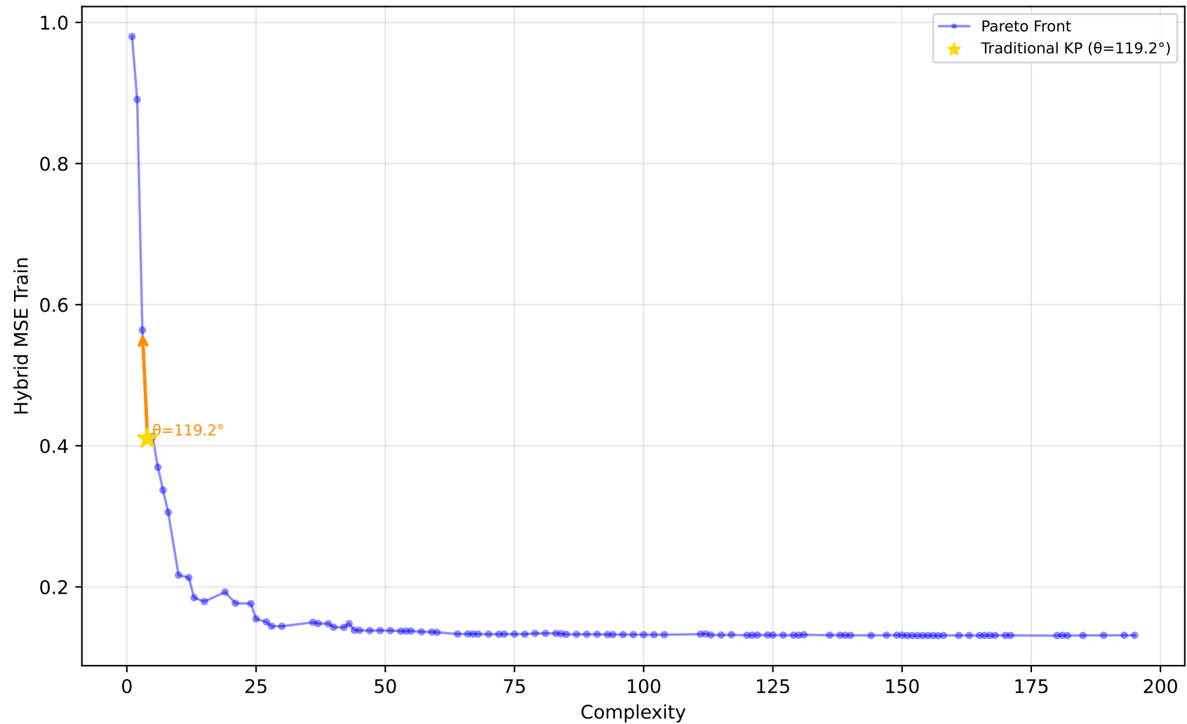
561_cpu - Run 14 - MVP - Hybrid MSE Train \lambda_1=0.70, \lambda_2=0.00, \lambda_3=0.10 | Difficulty: 1.00 | Method: hmr
