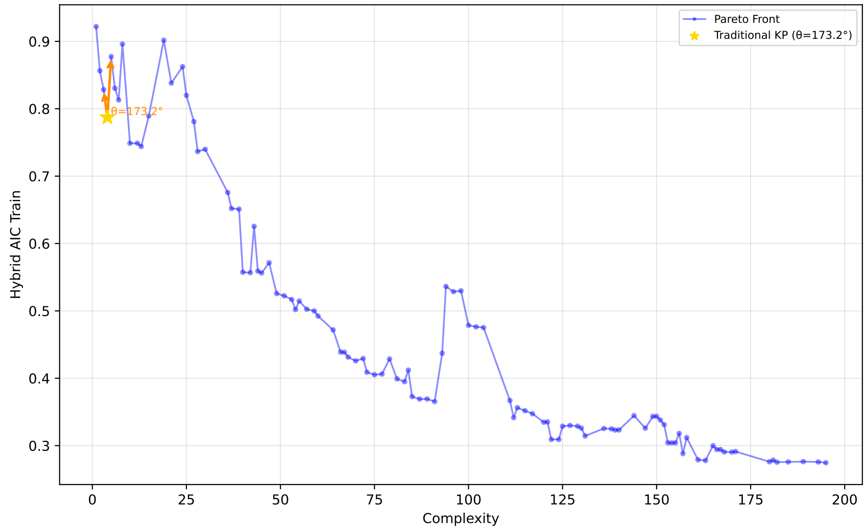
561_cpu - Run 14 - SVP - Hybrid AIC Train \lambda_1=0.90, \lambda_2=0.00, \lambda_3=0.30 | Difficulty: 1.00 | Method: hmr
