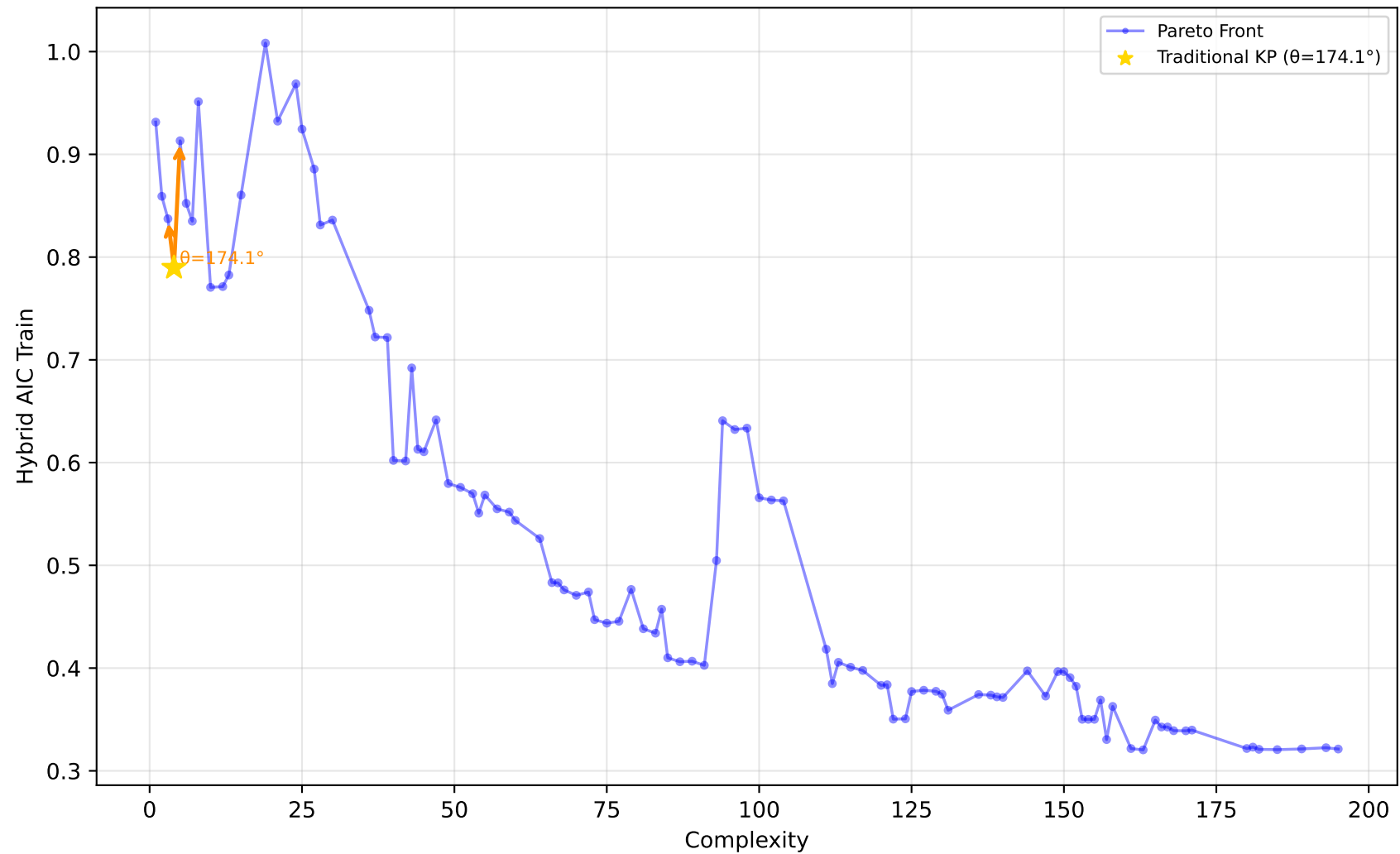
561_cpu - Run 14 - SVP - Hybrid AIC Train \lambda_1=1.00, \lambda_2=0.00, \lambda_3=0.40 | Difficulty: 1.00 | Method: hmr
