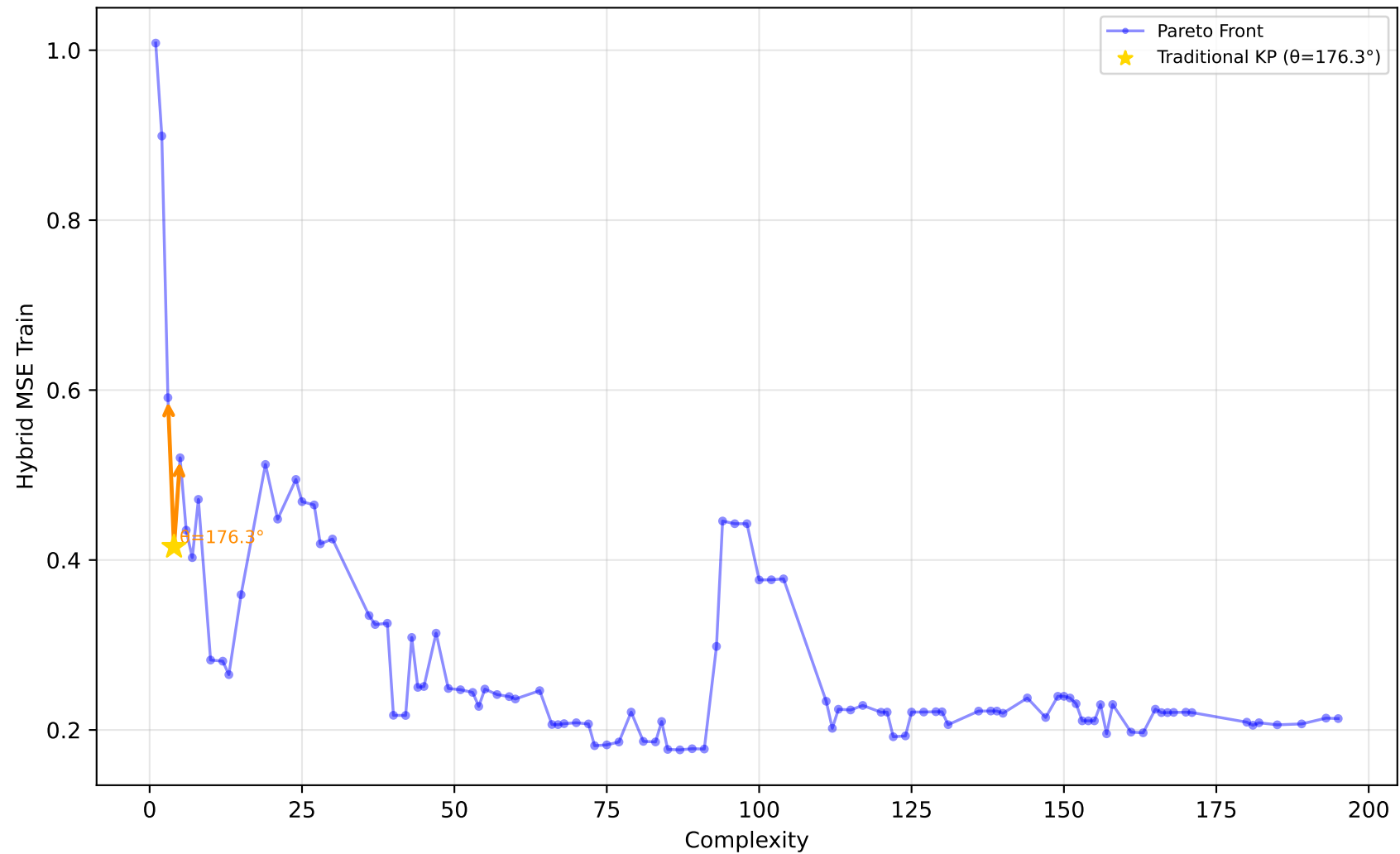
561_cpu - Run 14 - SVP - Hybrid MSE Train \lambda_1=1.00, \lambda_2=0.00, \lambda_3=0.40 | Difficulty: 1.00 | Method: hmr
