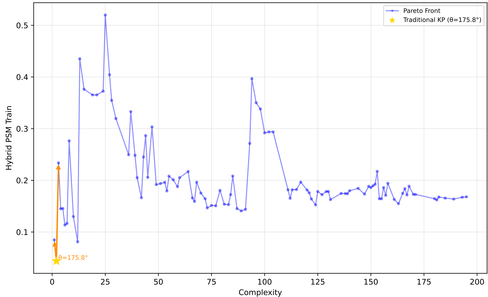
561_cpu - Run 14 - SVP - Hybrid PSM Train \lambda_1=0.90, \lambda_2=0.00, \lambda_3=0.30 | Difficulty: 1.00 | Method: hmr
