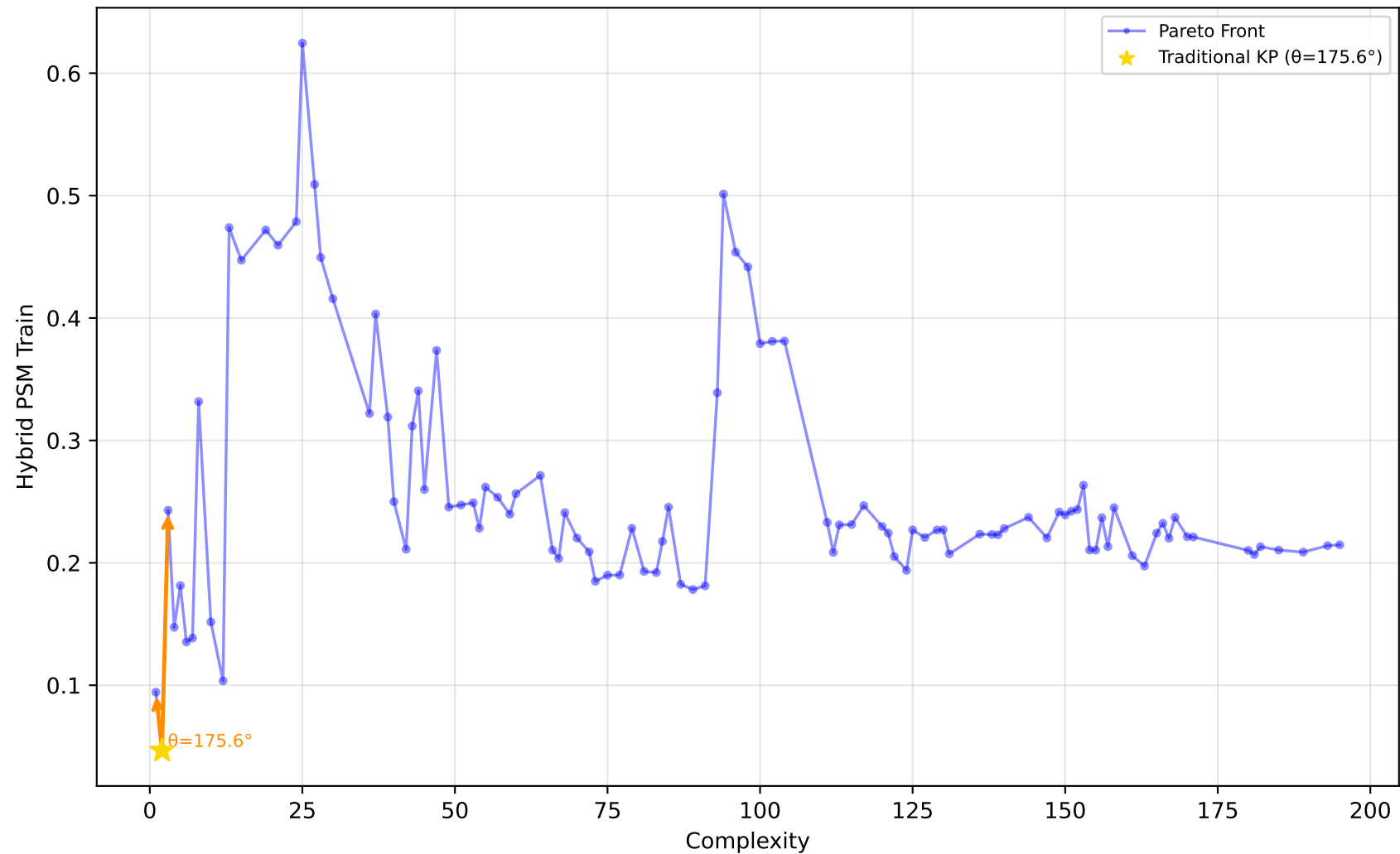
561_cpu - Run 14 - SVP - Hybrid PSM Train \lambda_1=1.00, \lambda_2=0.00, \lambda_3=0.40 | Difficulty: 1.00 | Method: hmr
