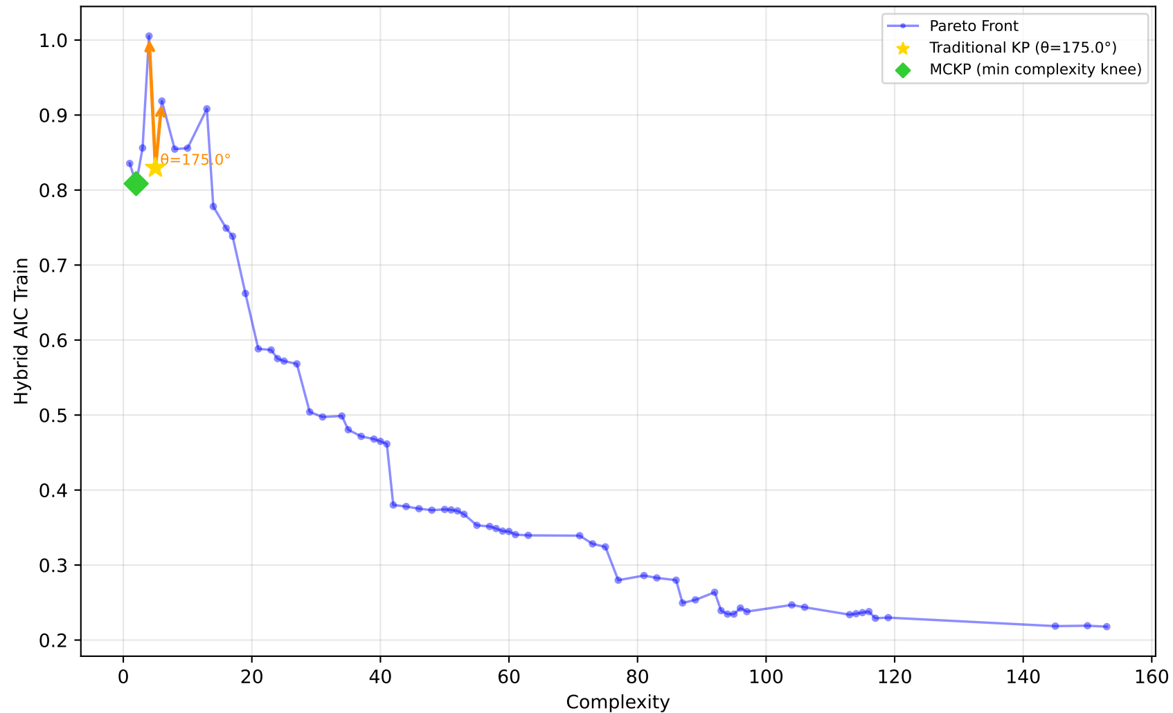
561_cpu - Run 15 - MVP - Hybrid AIC Train \lambda_1=0.70, \lambda_2=0.00, \lambda_3=0.10 | Difficulty: 1.00 | Method: hmr
