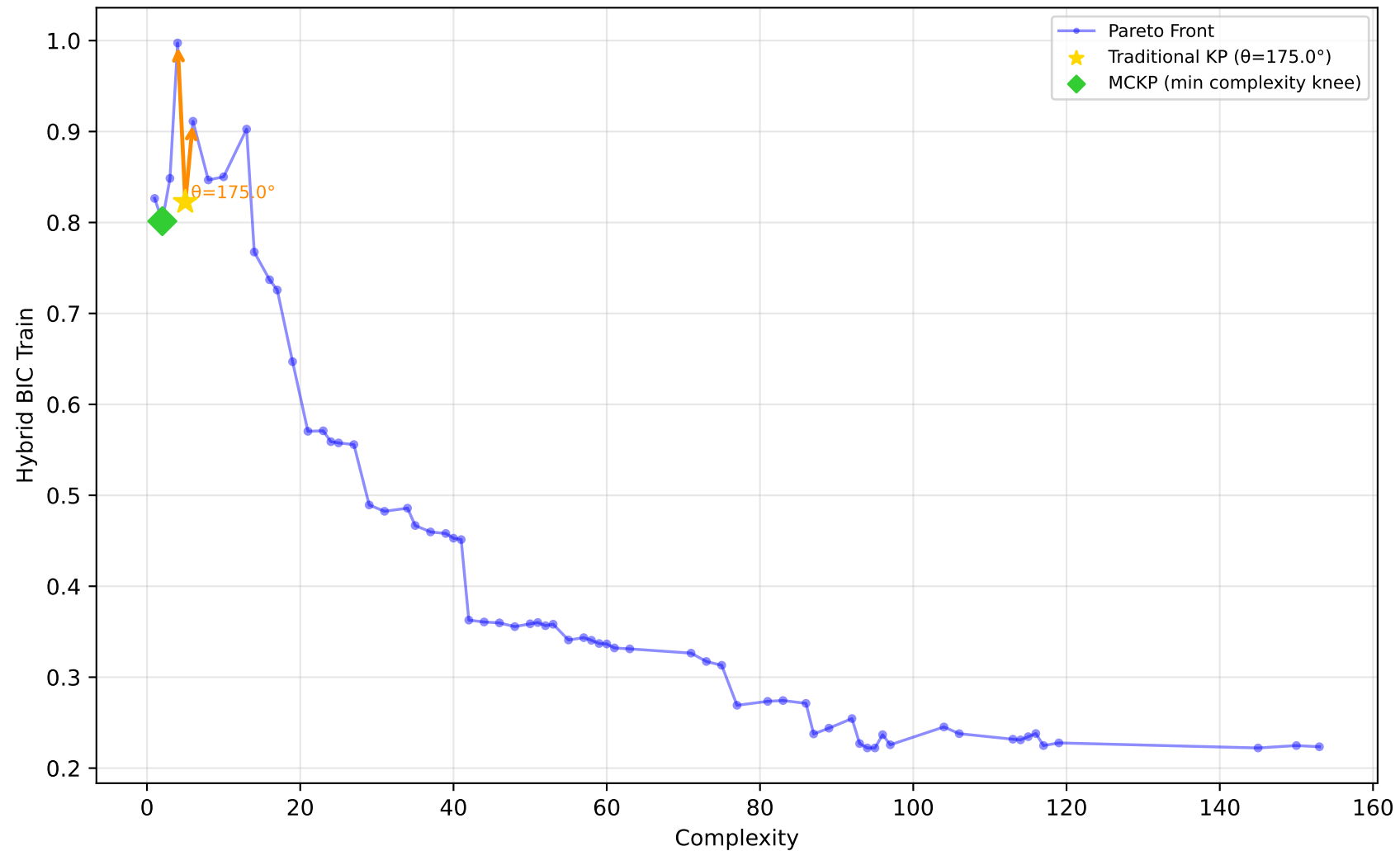
561_cpu - Run 15 - MVP - Hybrid BIC Train \lambda_1=0.70, \lambda_2=0.00, \lambda_3=0.10 | Difficulty: 1.00 | Method: hmr
