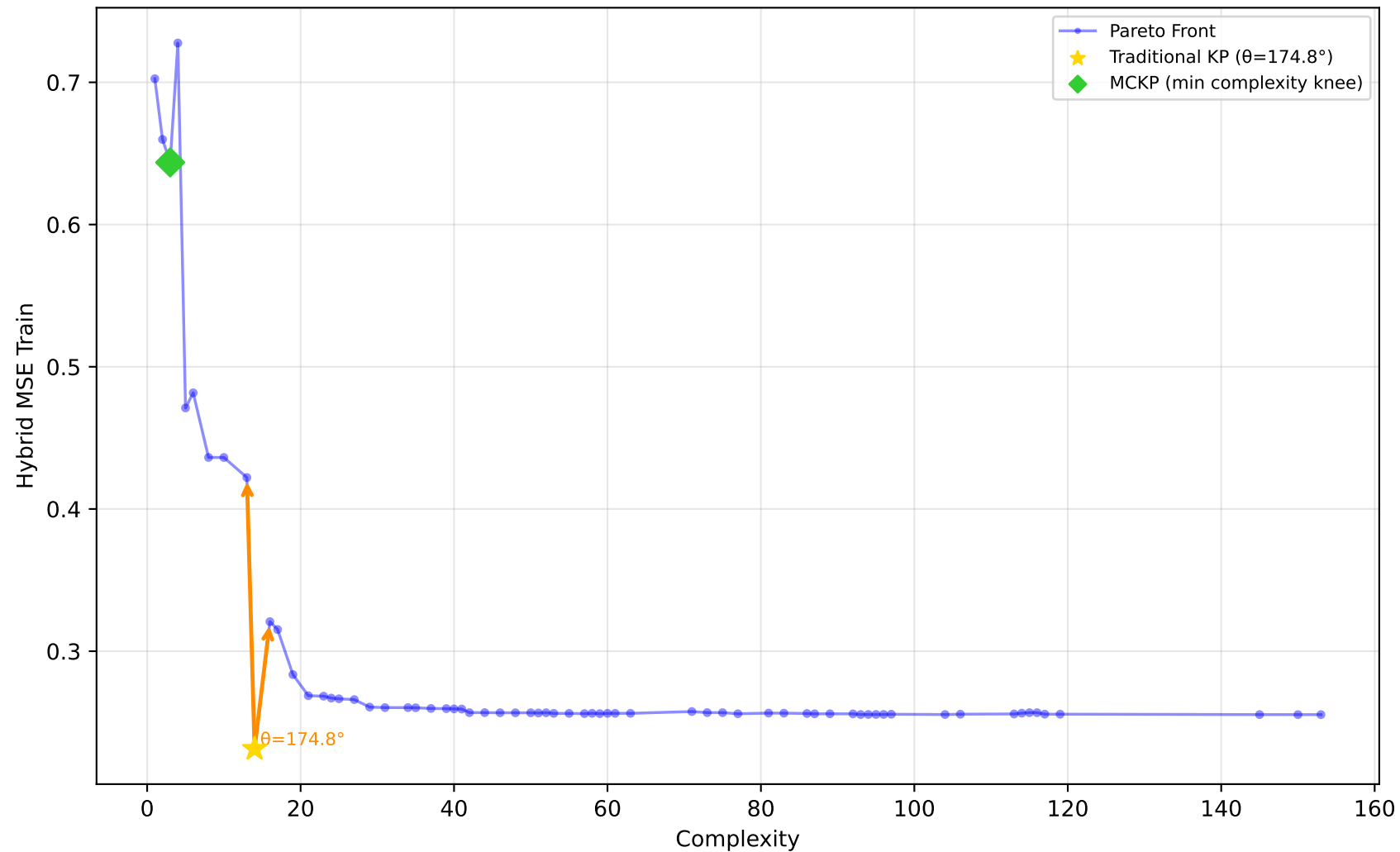
561_cpu - Run 15 - MVP - Hybrid MSE Train \lambda_1=0.50, \lambda_2=0.20, \lambda_3=0.00 | Difficulty: 1.00 | Method: hmr
