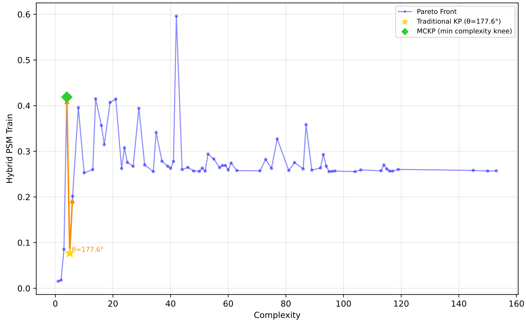
561_cpu - Run 15 - MVP - Hybrid PSM Train \lambda_1=0.50, \lambda_2=0.20, \lambda_3=0.00 | Difficulty: 1.00 | Method: hmr
