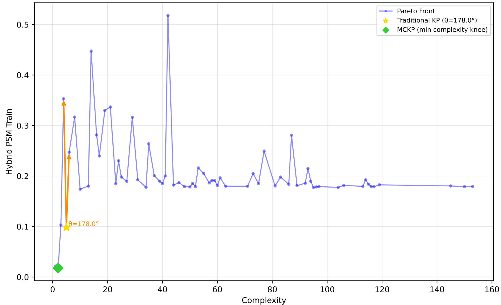
561_cpu - Run 15 - MVP - Hybrid PSM Train \lambda_1=0.70, \lambda_2=0.00, \lambda_3=0.10 | Difficulty: 1.00 | Method: hmr
