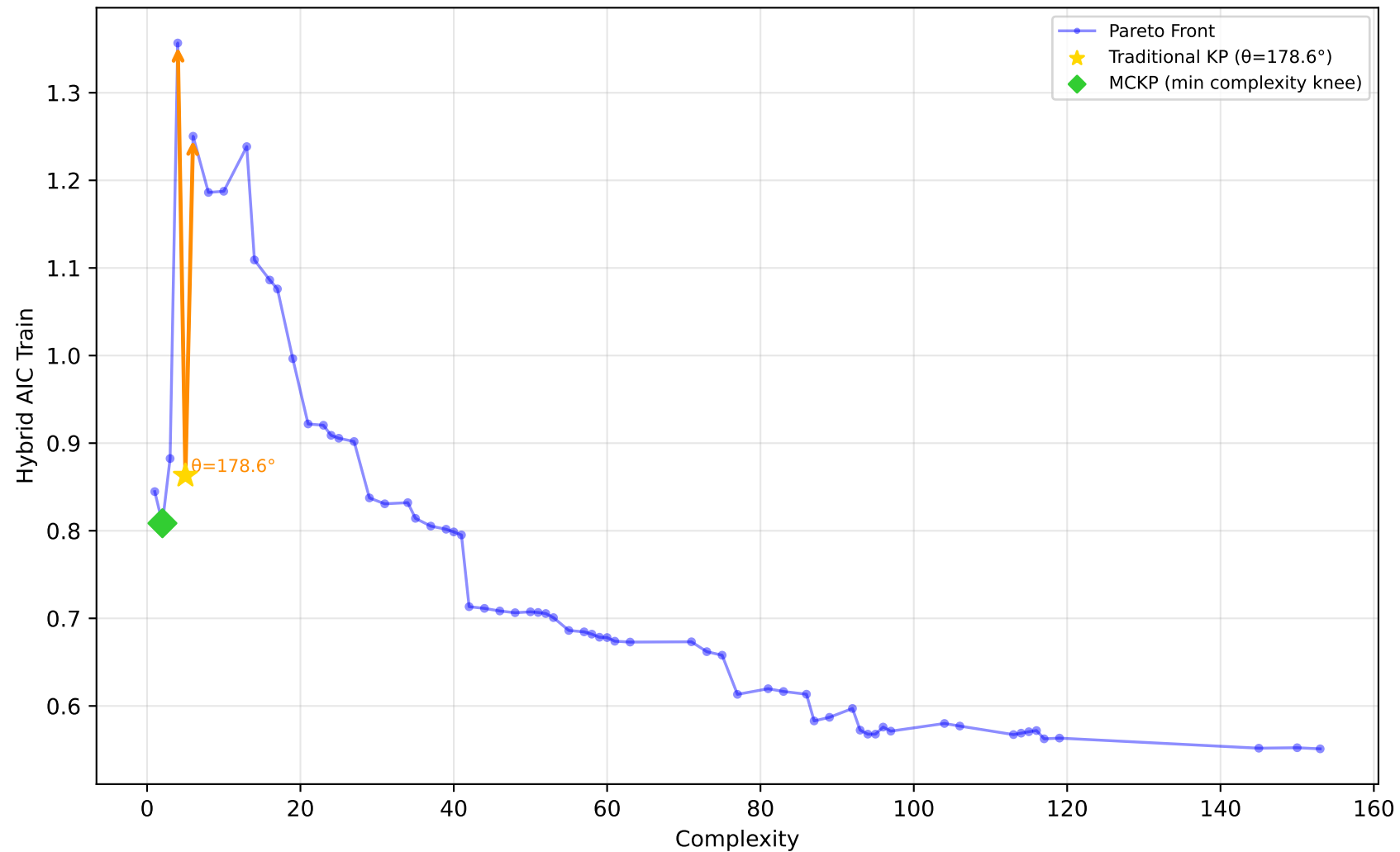
561_cpu - Run 15 - SVP - Hybrid AIC Train \lambda_1=1.00, \lambda_2=0.00, \lambda_3=0.40 | Difficulty: 1.00 | Method: hmr
