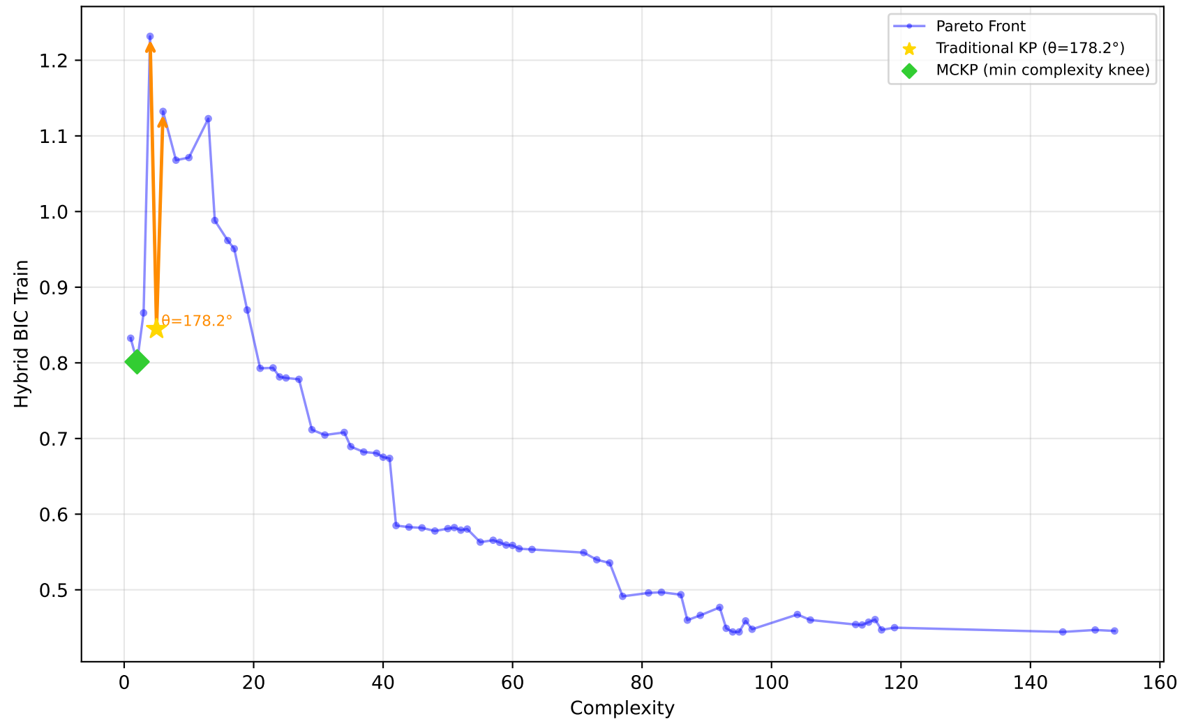
561_cpu - Run 15 - SVP - Hybrid BIC Train \lambda_1=0.90, \lambda_2=0.00, \lambda_3=0.30 | Difficulty: 1.00 | Method: hmr
