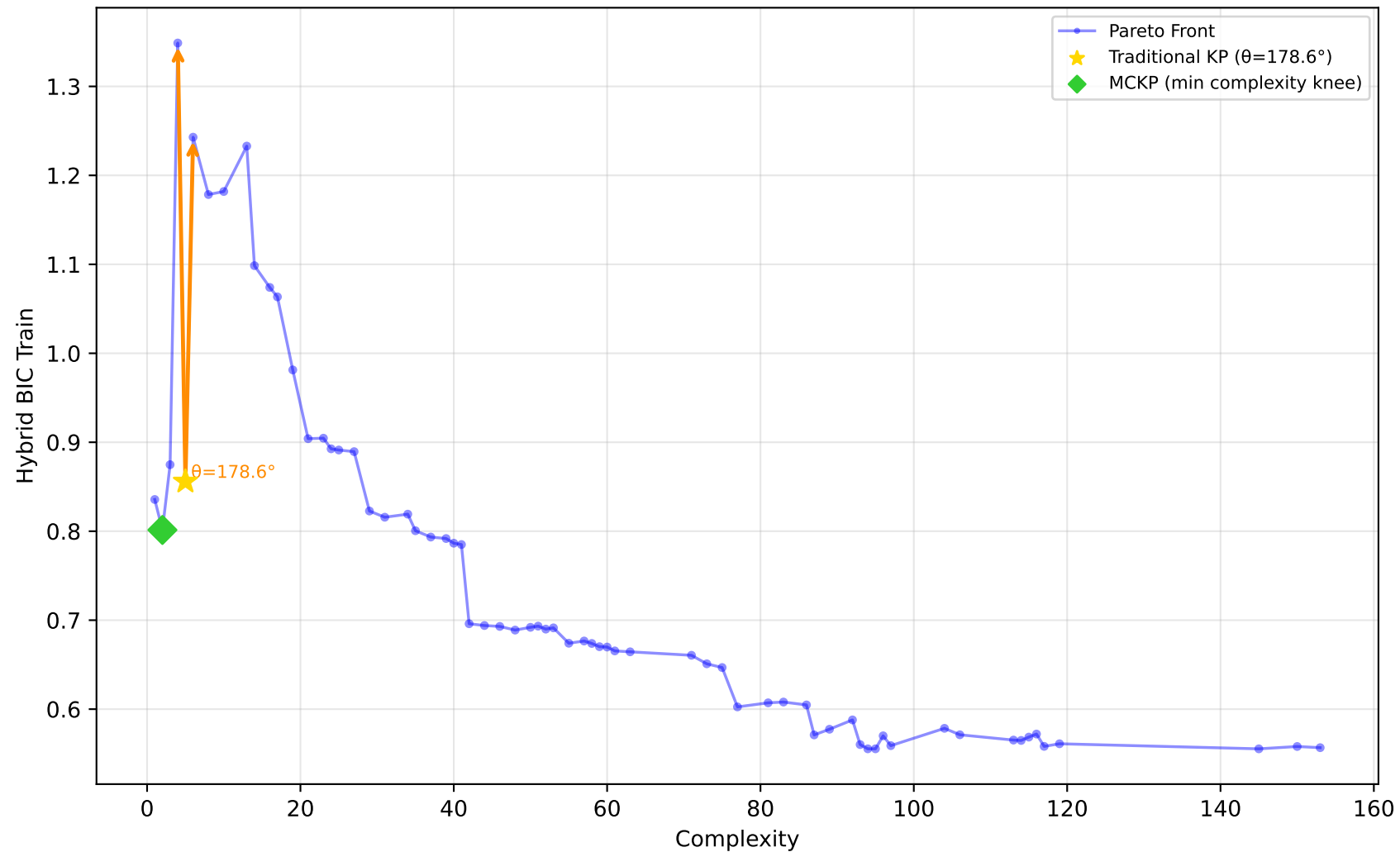
561_cpu - Run 15 - SVP - Hybrid BIC Train \lambda_1=1.00, \lambda_2=0.00, \lambda_3=0.40 | Difficulty: 1.00 | Method: hmr
