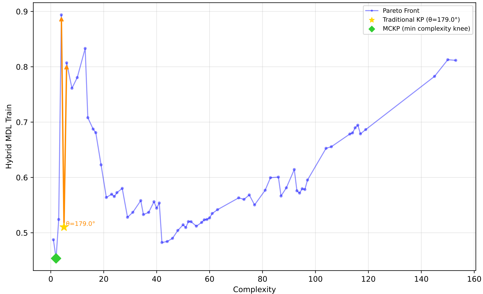
561_cpu - Run 15 - SVP - Hybrid MDL Train \lambda_1=0.90, \lambda_2=0.00, \lambda_3=0.30 | Difficulty: 1.00 | Method: hmr
