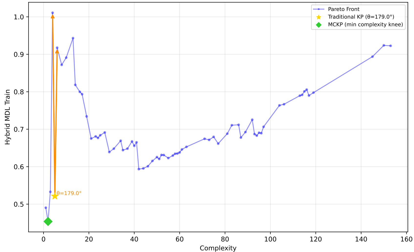
561_cpu - Run 15 - SVP - Hybrid MDL Train \lambda_1=1.00, \lambda_2=0.00, \lambda_3=0.40 | Difficulty: 1.00 | Method: hmr
