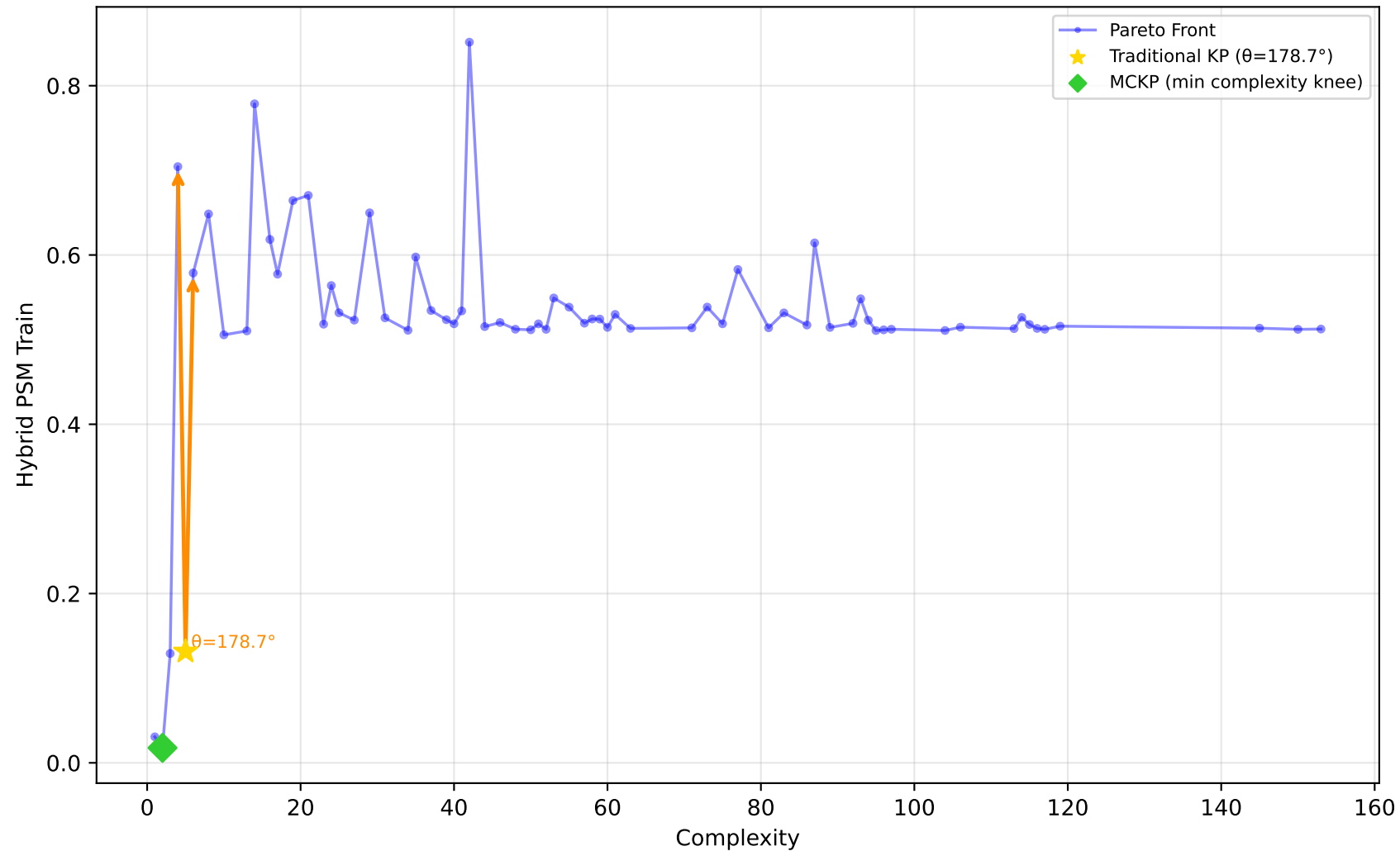
561_cpu - Run 15 - SVP - Hybrid PSM Train \lambda_1=1.00, \lambda_2=0.00, \lambda_3=0.40 | Difficulty: 1.00 | Method: hmr
