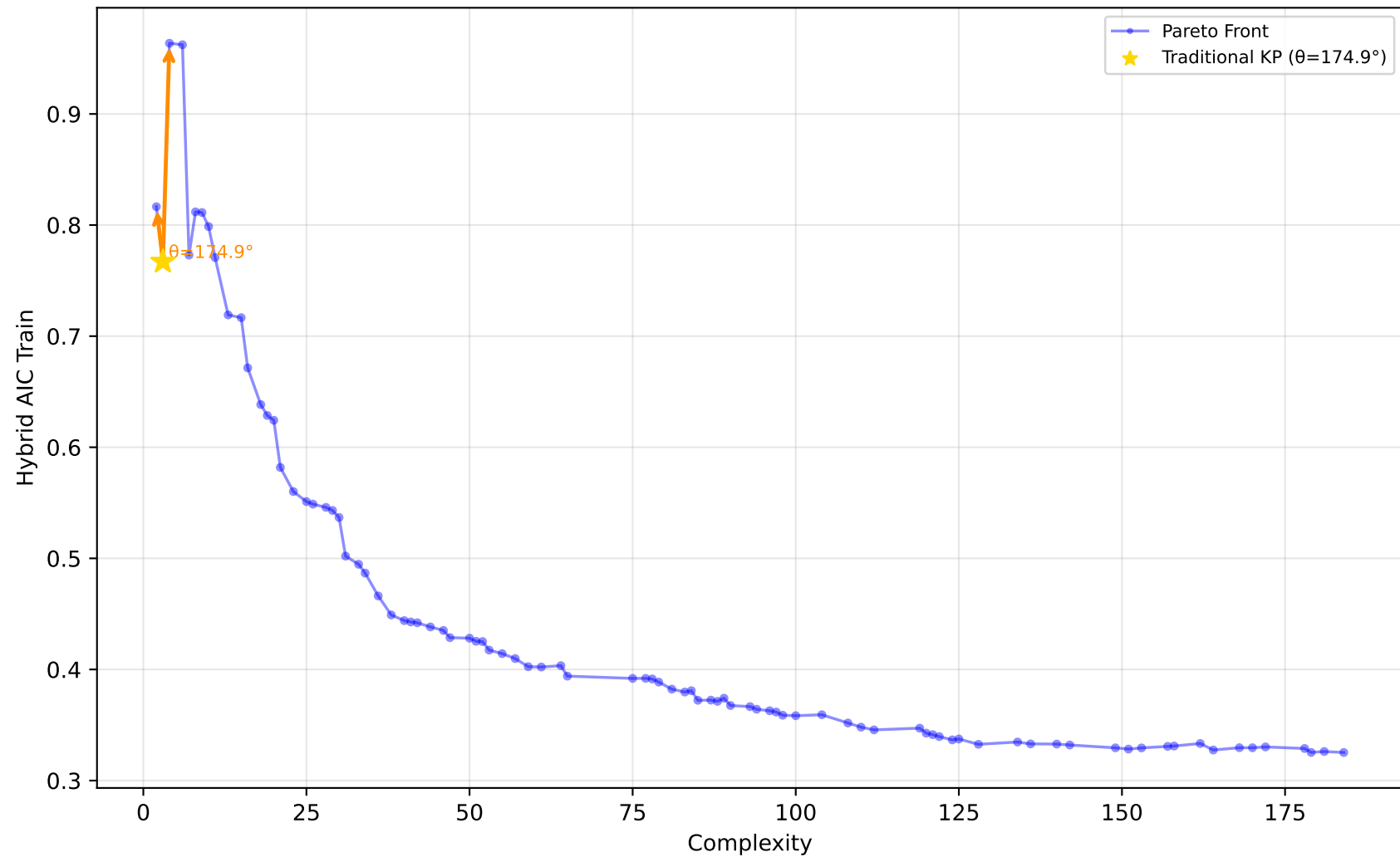
561_cpu - Run 16 - MVP - Hybrid AIC Train \lambda_1=0.50, \lambda_2=0.20, \lambda_3=0.00 | Difficulty: 0.94 | Method: hmr
