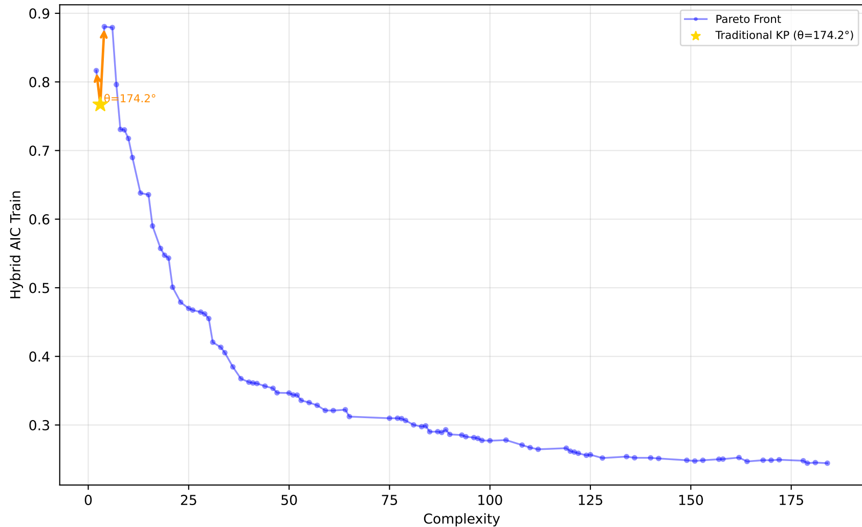
561_cpu - Run 16 - MVP - Hybrid AIC Train \lambda_1=0.70, \lambda_2=0.00, \lambda_3=0.10 | Difficulty: 0.94 | Method: hmr
