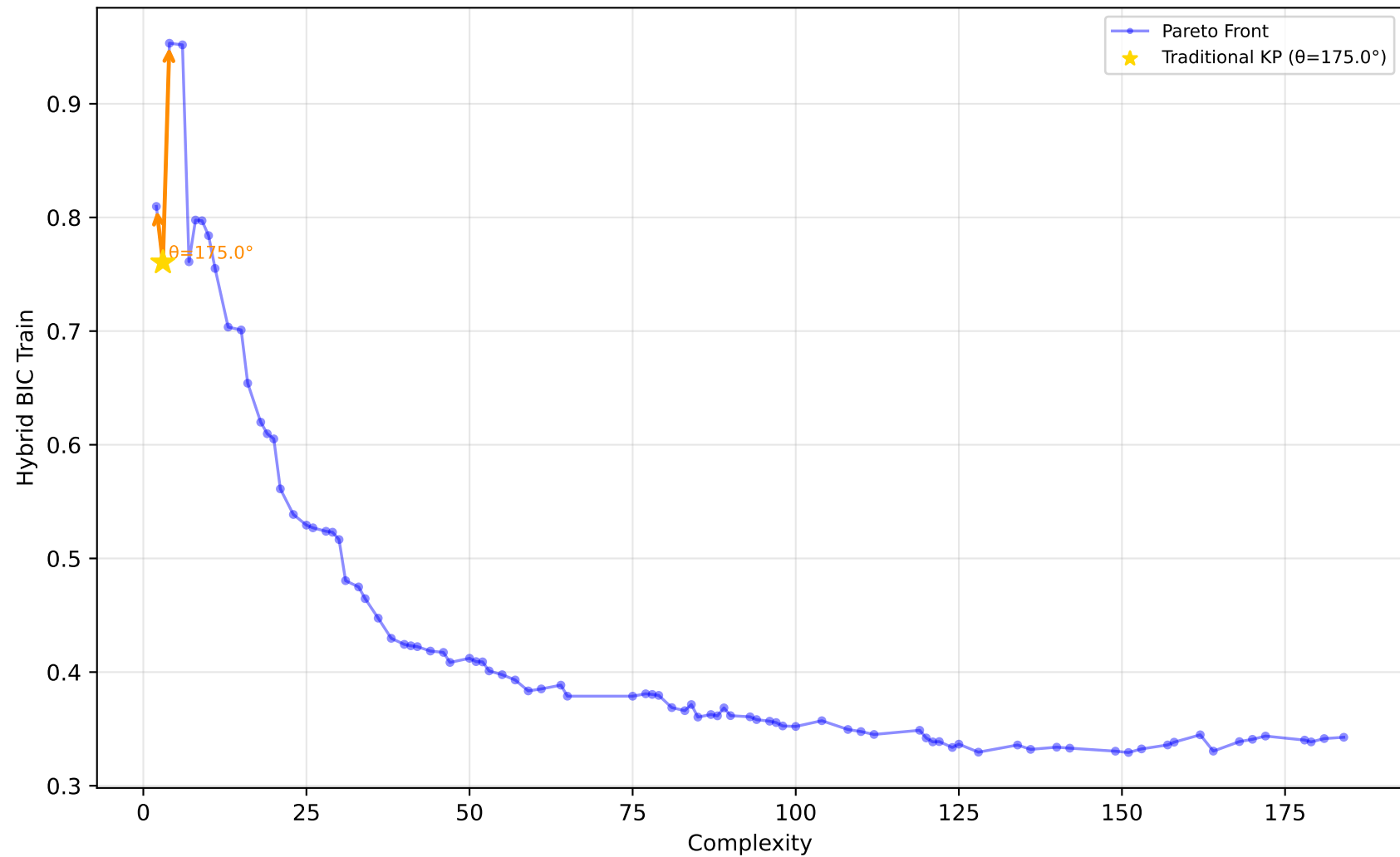
561_cpu - Run 16 - MVP - Hybrid BIC Train \lambda_1=0.50, \lambda_2=0.20, \lambda_3=0.00 | Difficulty: 0.94 | Method: hmr
