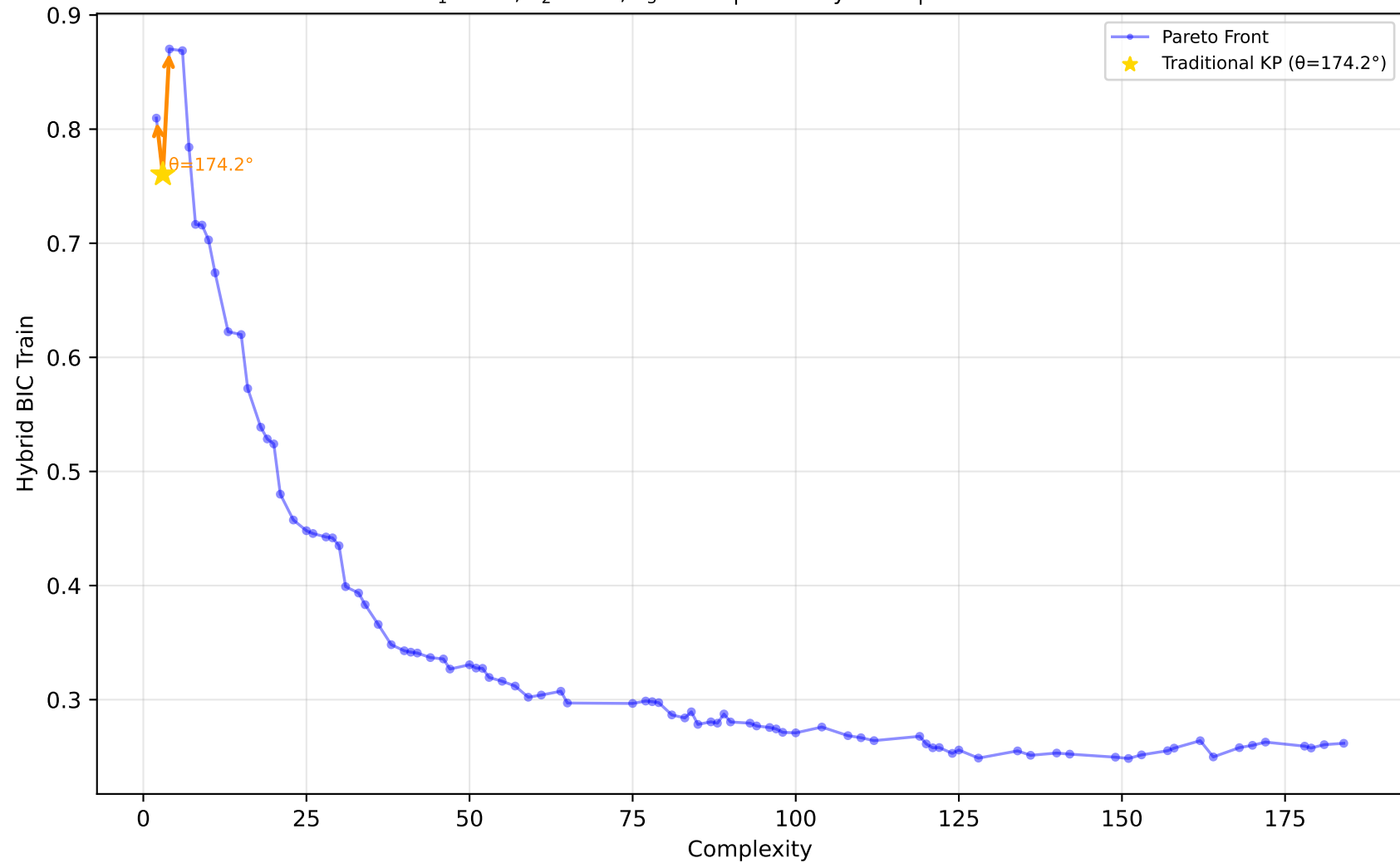
561_cpu - Run 16 - MVP - Hybrid BIC Train \lambda_1=0.70, \lambda_2=0.00, \lambda_3=0.10 | Difficulty: 0.94 | Method: hmr
